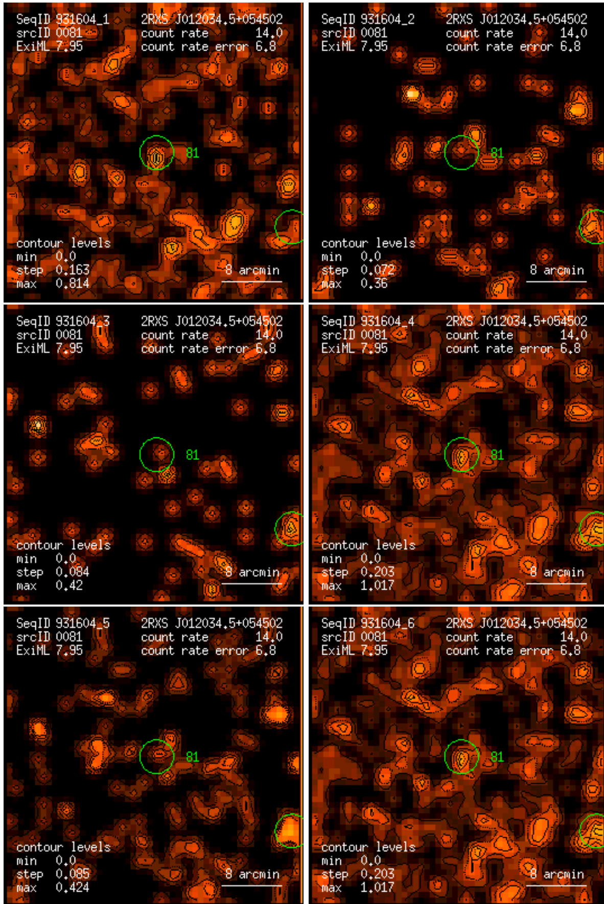
Figure 81: RASS 931604: detection 0081: band rate images, Gaussian filter: (1) PSPC channels 11 – 41, (2) 52 – 90, (3) 91 – 201, (4) 11 – 235, (5) 52 – 201, (6) 11 – 201. Broad band rates in counts/ks. Band rate contour levels in counts/ks/arcmin 2 .
