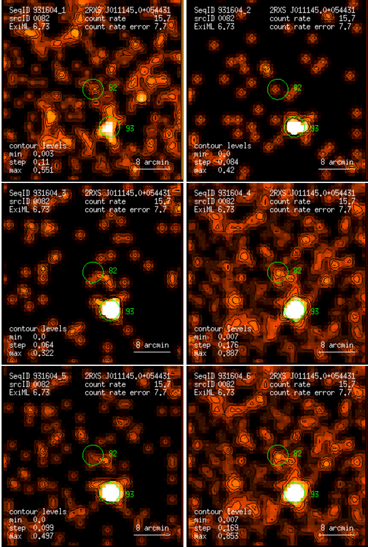
Figure 82: RASS 931604: detection 0082: band rate images, Gaussian filter: (1) PSPC channels 11 – 41, (2) 52 – 90, (3) 91 – 201, (4) 11 – 235, (5) 52 – 201, (6) 11 – 201. Broad band rates in counts/ks. Band rate contour levels in counts/ks/arcmin 2 .
