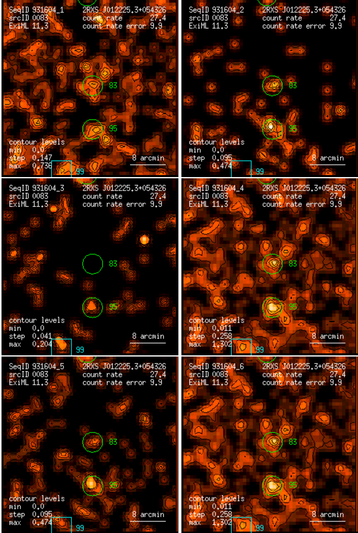
Figure 83: RASS 931604: detection 0083: band rate images, Gaussian filter: (1) PSPC channels 11 – 41, (2) 52 – 90, (3) 91 – 201, (4) 11 – 235, (5) 52 – 201, (6) 11 – 201. Broad band rates in counts/ks. Band rate contour levels in counts/ks/arcmin 2 .
