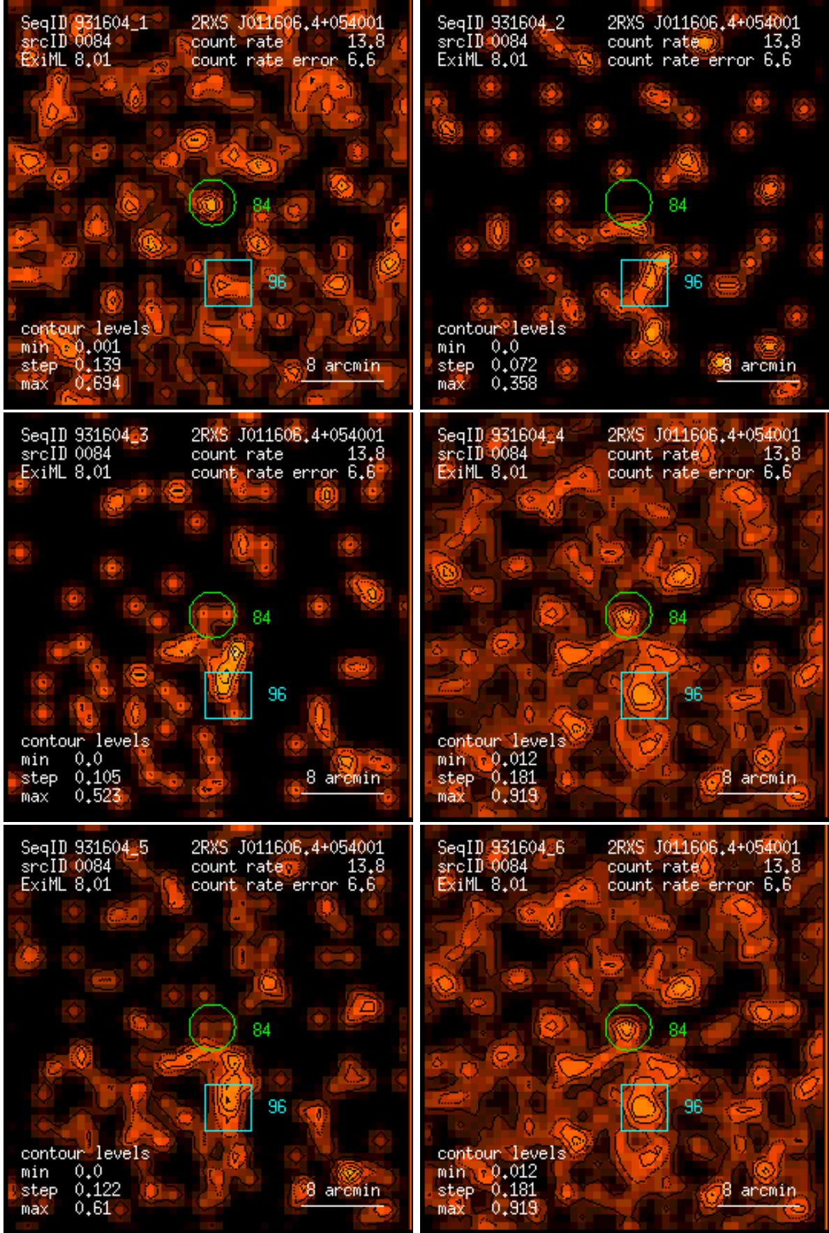
Figure 84: RASS 931604: detection 0084: band rate images, Gaussian filter: (1) PSPC channels 11 – 41, (2) 52 – 90, (3) 91 – 201, (4) 11 – 235, (5) 52 – 201, (6) 11 – 201. Broad band rates in counts/ks. Band rate contour levels in counts/ks/arcmin 2 .
