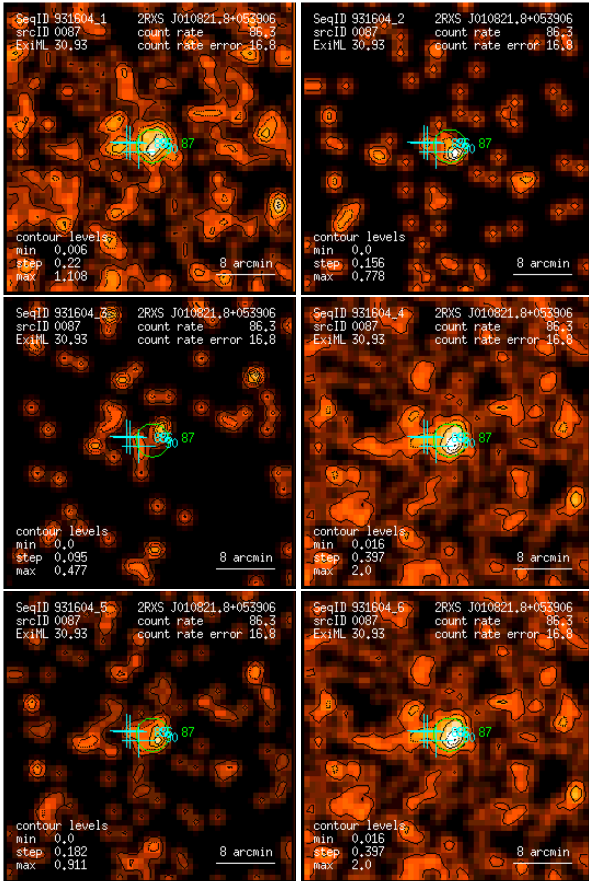
Figure 87: RASS 931604: detection 0087: band rate images, Gaussian filter: (1) PSPC channels 11 – 41, (2) 52 – 90, (3) 91 – 201, (4) 11 – 235, (5) 52 – 201, (6) 11 – 201. Broad band rates in counts/ks. Band rate contour levels in counts/ks/arcmin 2 .
