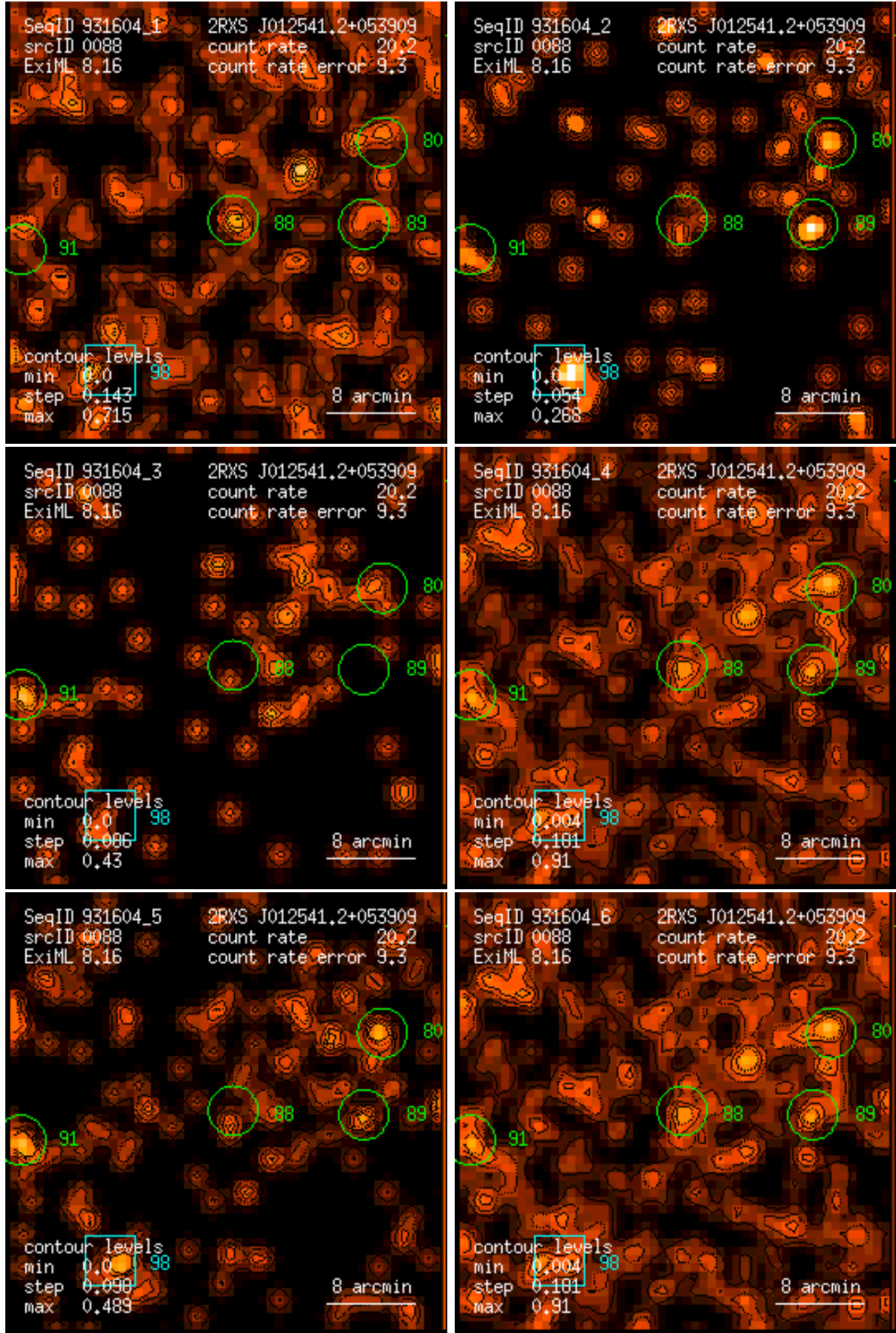
Figure 88: RASS 931604: detection 0088: band rate images, Gaussian filter: (1) PSPC channels 11 – 41, (2) 52 – 90, (3) 91 – 201, (4) 11 – 235, (5) 52 – 201, (6) 11 – 201. Broad band rates in counts/ks. Band rate contour levels in counts/ks/arcmin 2 .
