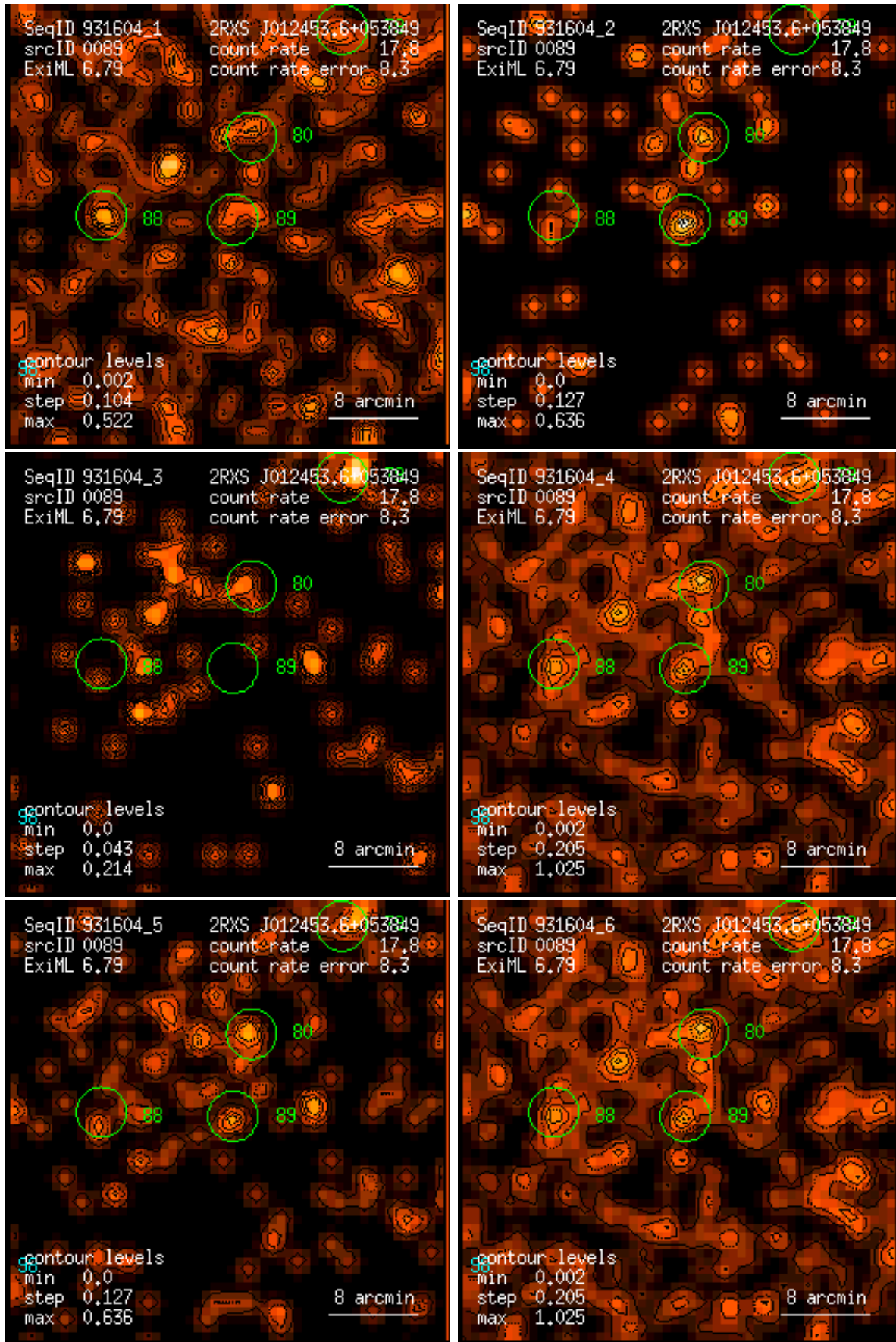
Figure 89: RASS 931604: detection 0089: band rate images, Gaussian filter: (1) PSPC channels 11 – 41, (2) 52 – 90, (3) 91 – 201, (4) 11 – 235, (5) 52 – 201, (6) 11 – 201. Broad band rates in counts/ks. Band rate contour levels in counts/ks/arcmin 2 .
