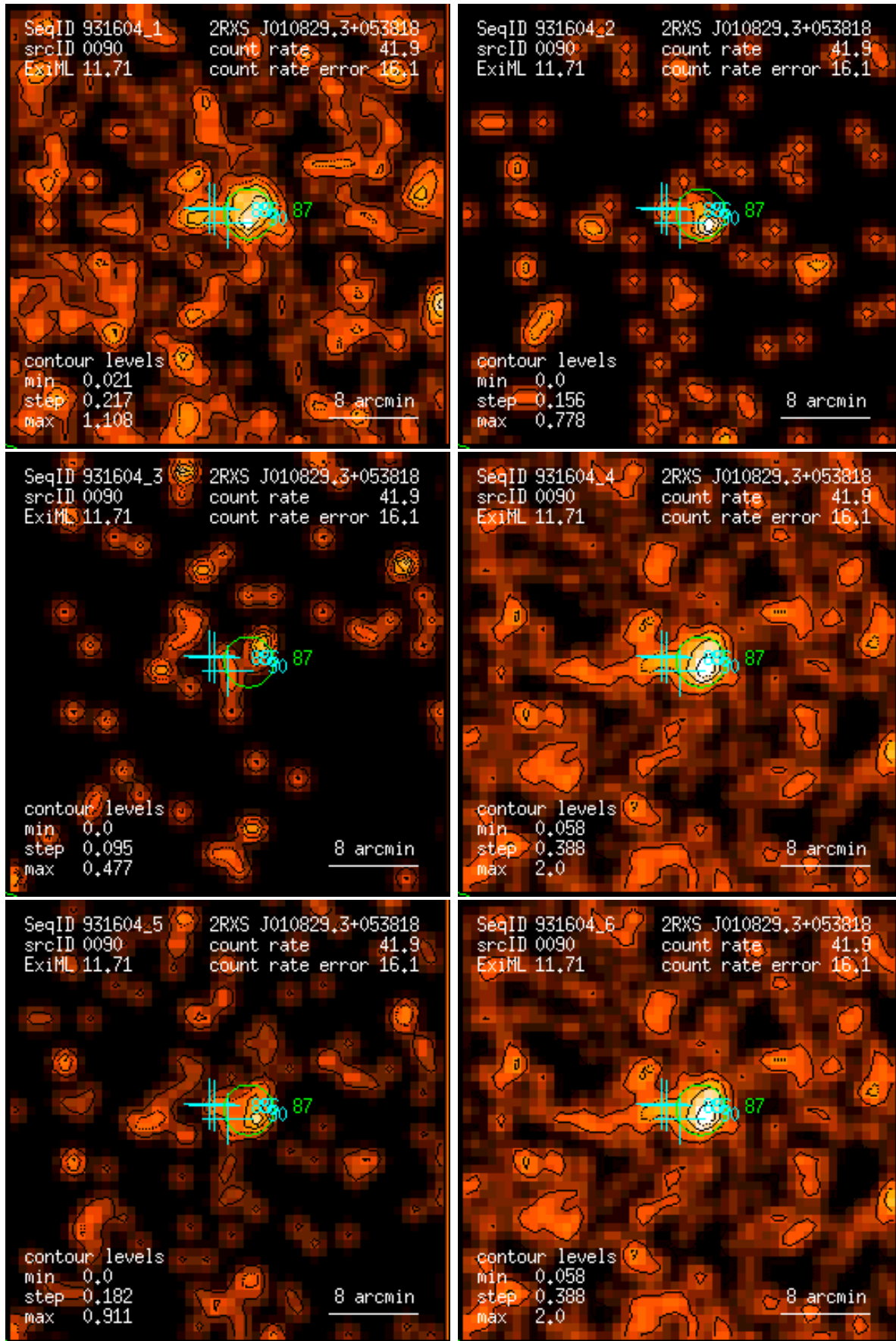
Figure 90: RASS 931604: detection 0090: band rate images, Gaussian filter: (1) PSPC channels 11 – 41, (2) 52 – 90, (3) 91 – 201, (4) 11 – 235, (5) 52 – 201, (6) 11 – 201. Broad band rates in counts/ks. Band rate contour levels in counts/ks/arcmin 2 .
