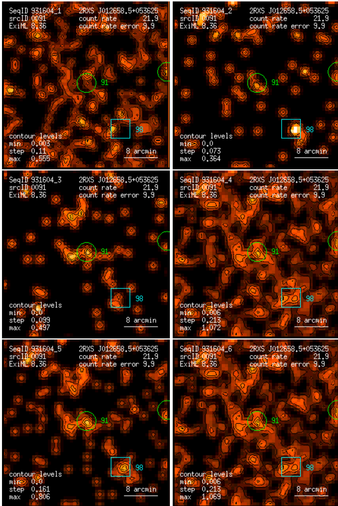
Figure 91: RASS 931604: detection 0091: band rate images, Gaussian filter: (1) PSPC channels 11 – 41, (2) 52 – 90, (3) 91 – 201, (4) 11 – 235, (5) 52 – 201, (6) 11 – 201. Broad band rates in counts/ks. Band rate contour levels in counts/ks/arcmin 2 .
