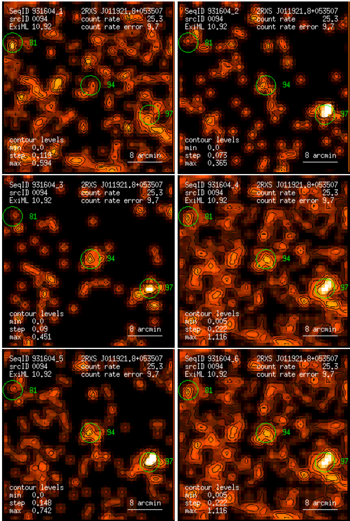
Figure 94: RASS 931604: detection 0094: band rate images, Gaussian filter: (1) PSPC channels 11 – 41, (2) 52 – 90, (3) 91 – 201, (4) 11 – 235, (5) 52 – 201, (6) 11 – 201. Broad band rates in counts/ks. Band rate contour levels in counts/ks/arcmin 2 .
