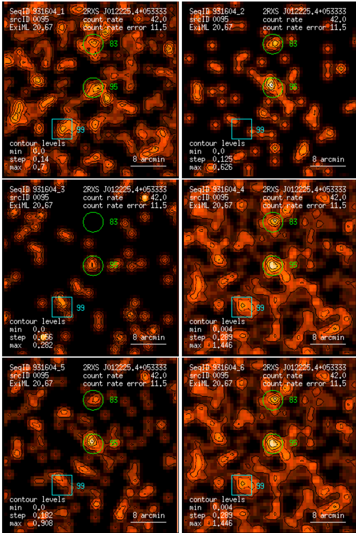
Figure 95: RASS 931604: detection 0095: band rate images, Gaussian filter: (1) PSPC channels 11 – 41, (2) 52 – 90, (3) 91 – 201, (4) 11 – 235, (5) 52 – 201, (6) 11 – 201. Broad band rates in counts/ks. Band rate contour levels in counts/ks/arcmin 2 .
