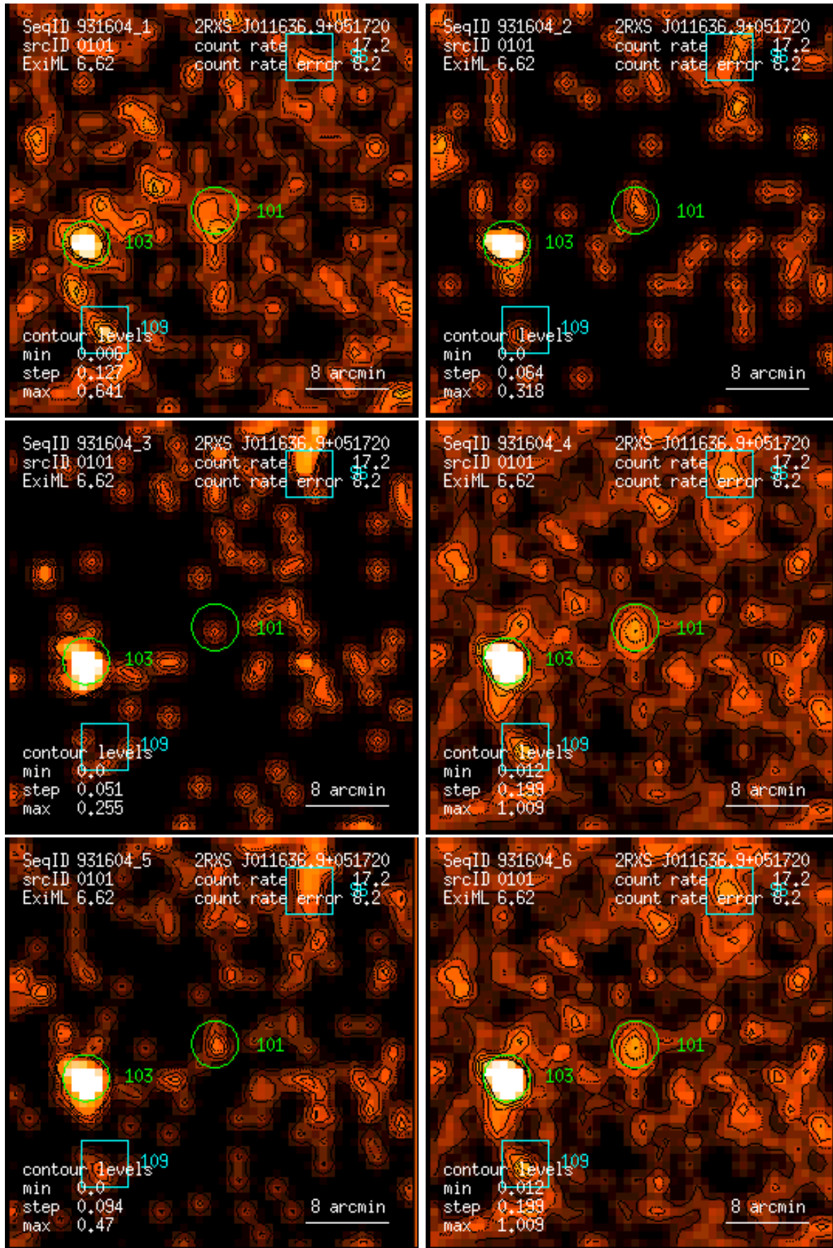
Figure 101: RASS 931604: detection 0101: band rate images, Gaussian filter: (1) PSPC channels 11 – 41, (2) 52 – 90, (3) 91 – 201, (4) 11 – 235, (5) 52 – 201, (6) 11 – 201. Broad band rates in counts/ks. Band rate contour levels in counts/ks/arcmin 2 .
