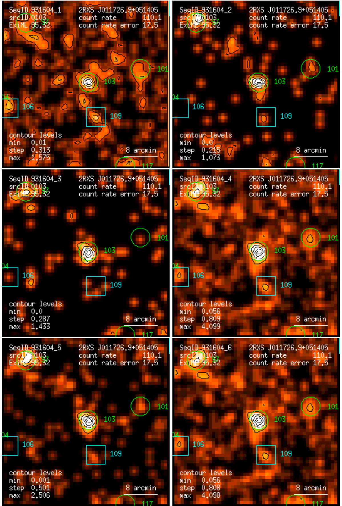
Figure 103: RASS 931604: detection 0103: band rate images, Gaussian filter: (1) PSPC channels 11 – 41, (2) 52 – 90, (3) 91 – 201, (4) 11 – 235, (5) 52 – 201, (6) 11 – 201. Broad band rates in counts/ks. Band rate contour levels in counts/ks/arcmin 2 .
