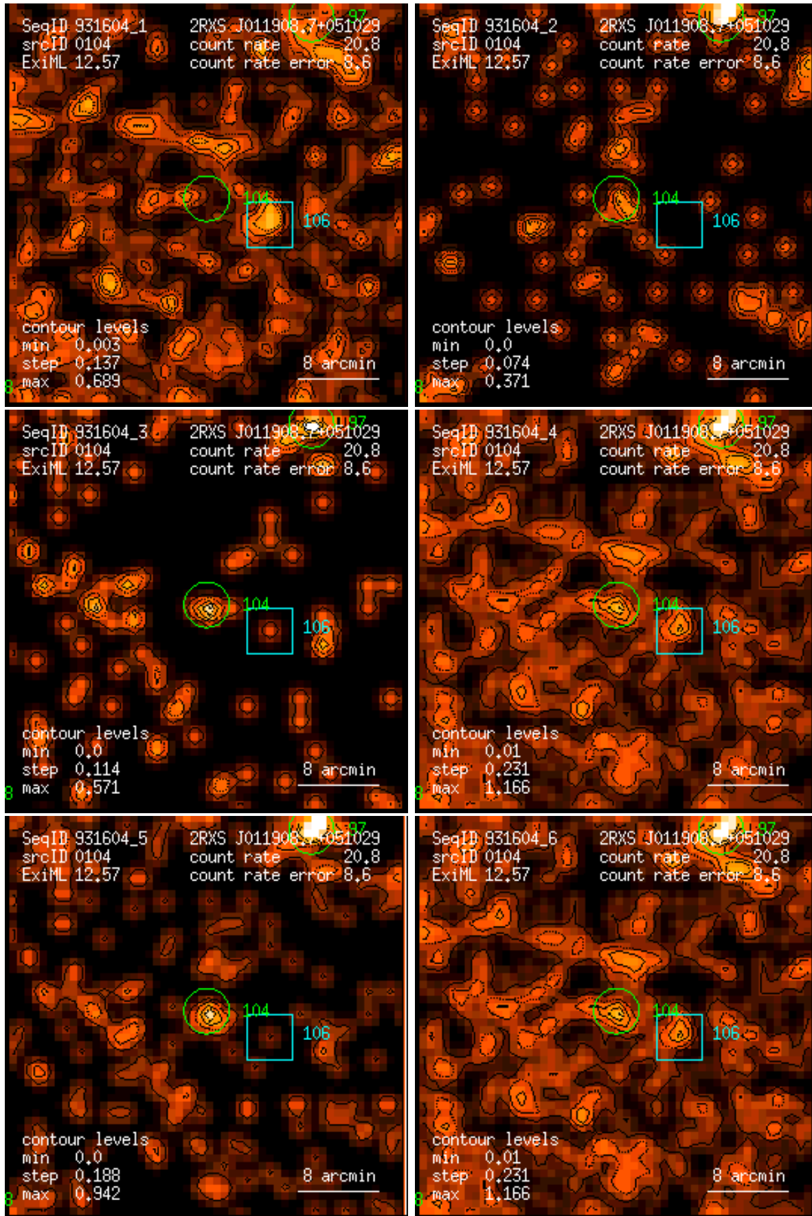
Figure 104: RASS 931604: detection 0104: band rate images, Gaussian filter: (1) PSPC channels 11 – 41, (2) 52 – 90, (3) 91 – 201, (4) 11 – 235, (5) 52 – 201, (6) 11 – 201. Broad band rates in counts/ks. Band rate contour levels in counts/ks/arcmin 2 .
