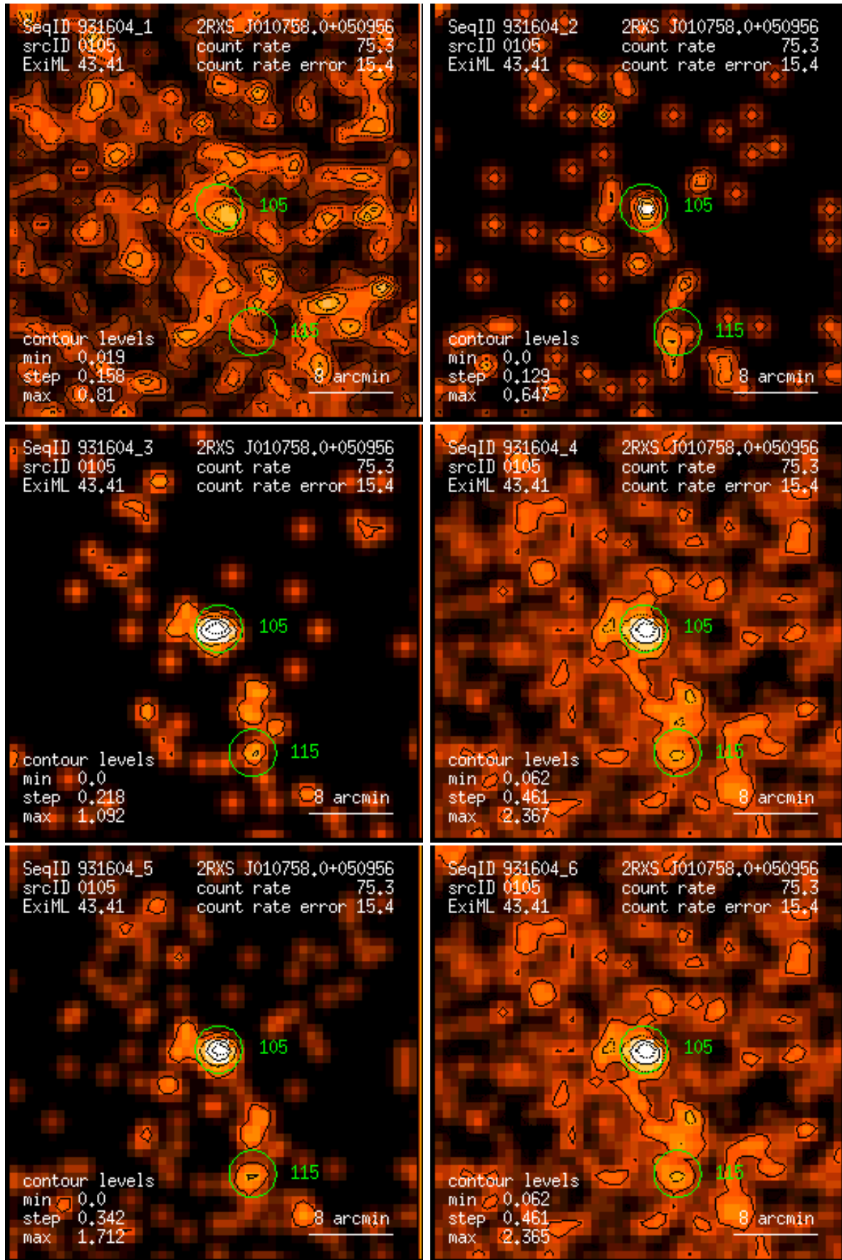
Figure 105: RASS 931604: detection 0105: band rate images, Gaussian filter: (1) PSPC channels 11 – 41, (2) 52 – 90, (3) 91 – 201, (4) 11 – 235, (5) 52 – 201, (6) 11 – 201. Broad band rates in counts/ks. Band rate contour levels in counts/ks/arcmin 2 .
