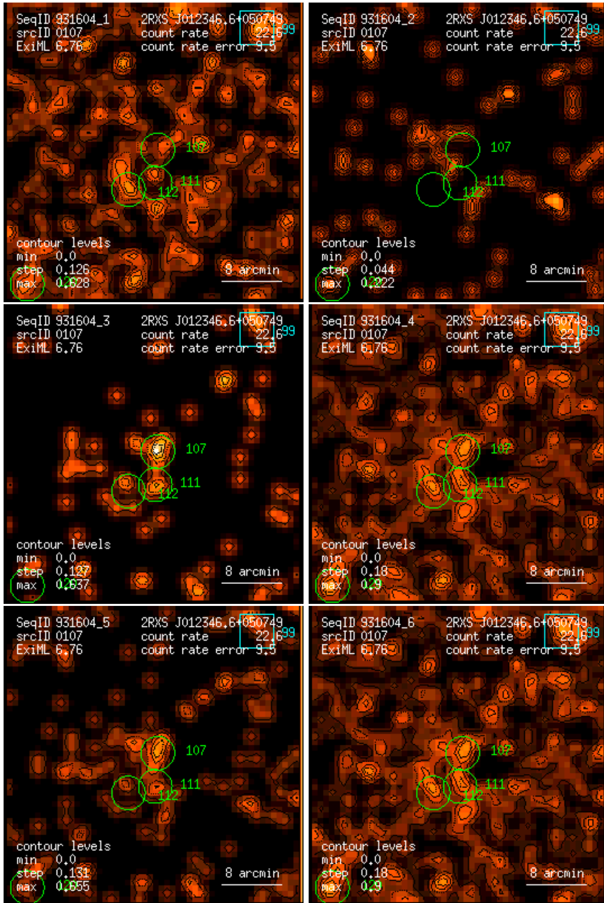
Figure 107: RASS 931604: detection 0107: band rate images, Gaussian filter: (1) PSPPC channels 11 – 41, (2) 52 – 90, (3) 91 – 201, (4) 11 – 235, (5) 52 – 201, (6) 11 – 201. Broad band rates in counts/ks. Band rate contour levels in counts/ks/arcmin 2 .
