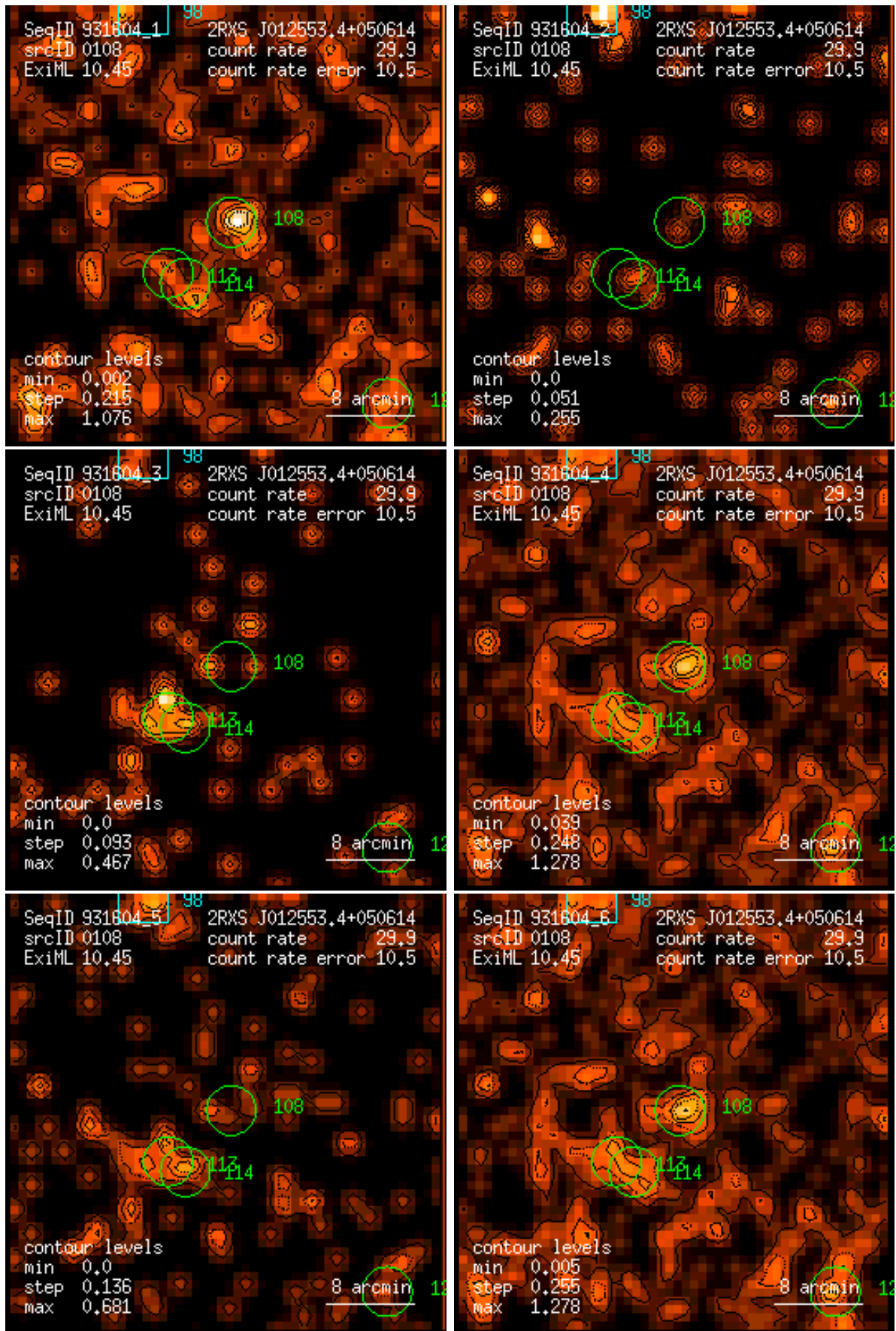
Figure 108: RASS 931604: detection 0108: band rate images, Gaussian filter: (1) PSPC channels 11 – 41, (2) 52 – 90, (3) 91 – 201, (4) 11 – 235, (5) 52 – 201, (6) 11 – 201. Broad band rates in counts/ks. Band rate contour levels in counts/ks/arcmin 2 .
