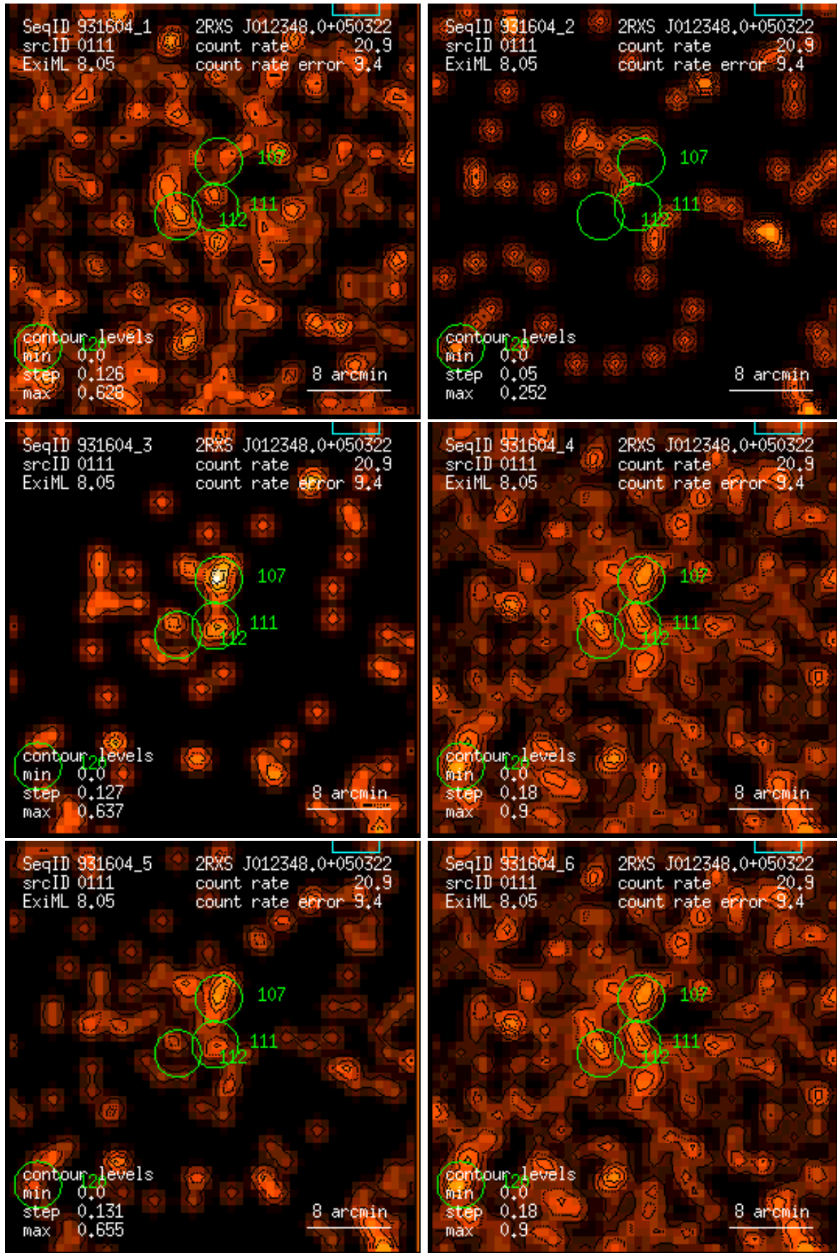
Figure 111: RASS 931604: detection 0111: band rate images, Gaussian filter: (1) PSPC channels 11 – 41, (2) 52 – 90, (3) 91 – 201, (4) 11 – 235, (5) 52 – 201, (6) 11 – 201. Broad band rates in counts/ks. Band rate contour levels in counts/ks/arcmin 2 .
