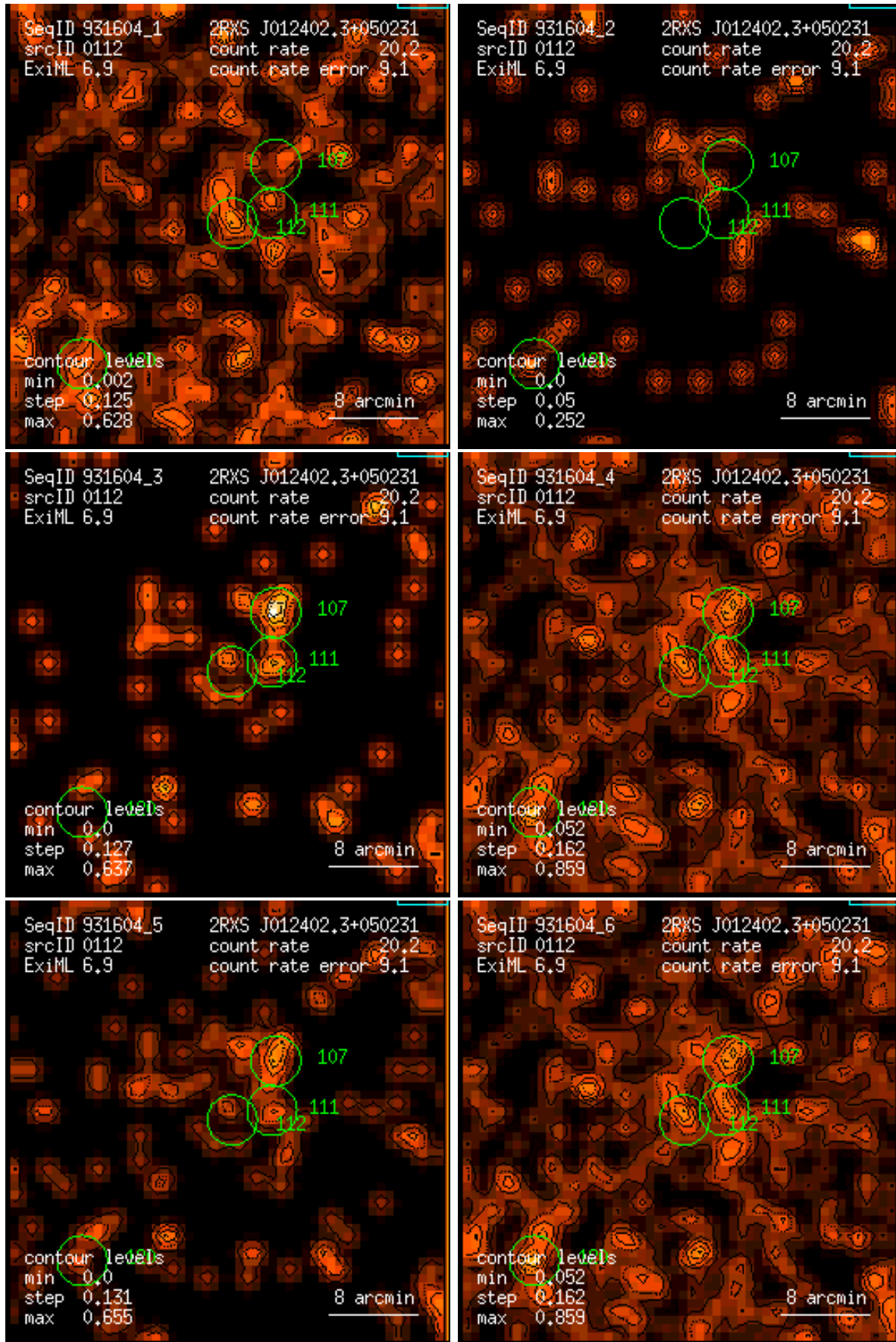
Figure 112: RASS 931604: detection 0112: band rate images, Gaussian filter: (1) PSPC channels 11 – 41, (2) 52 – 90, (3) 91 – 201, (4) 11 – 235, (5) 52 – 201, (6) 11 – 201. Broad band rates in counts/ks. Band rate contour levels in counts/ks/arcmin 2 .
