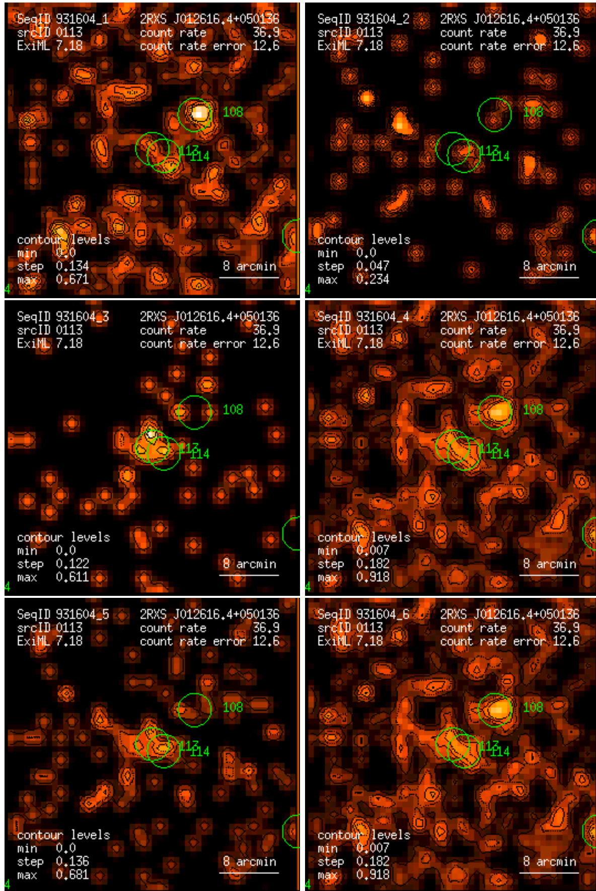
Figure 113: RASS 931604: detection 0113: band rate images, Gaussian filter: (1) PSPC channels 11 – 41, (2) 52 – 90, (3) 91 – 201, (4) 11 – 235, (5) 52 – 201, (6) 11 – 201. Broad band rates in counts/ks. Band rate contour levels in counts/ks/arcmin 2 .
