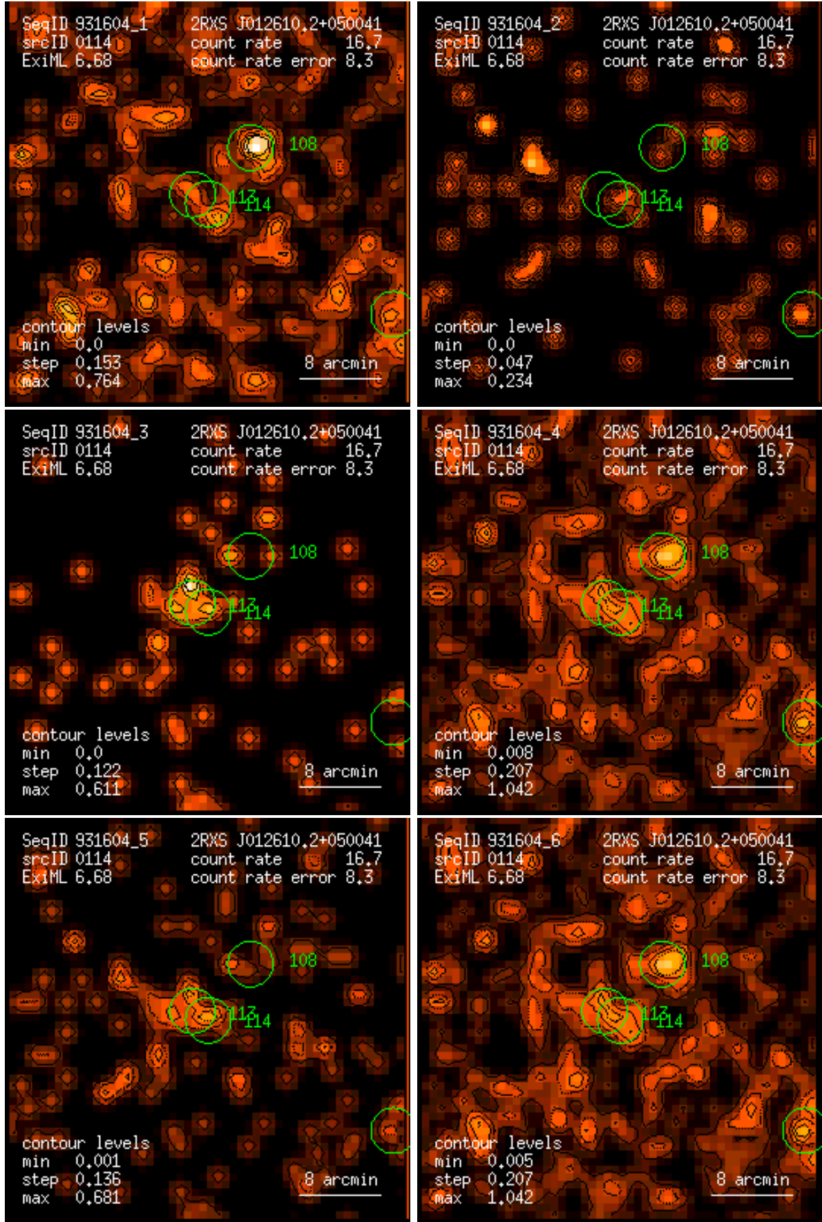
Figure 114: RASS 931604: detection 0114: band rate images, Gaussian filter: (1) PSPC channels 11 – 41, (2) 52 – 90, (3) 91 – 201, (4) 11 – 235, (5) 52 – 201, (6) 11 – 201. Broad band rates in counts/ks. Band rate contour levels in counts/ks/arcmin 2 .
