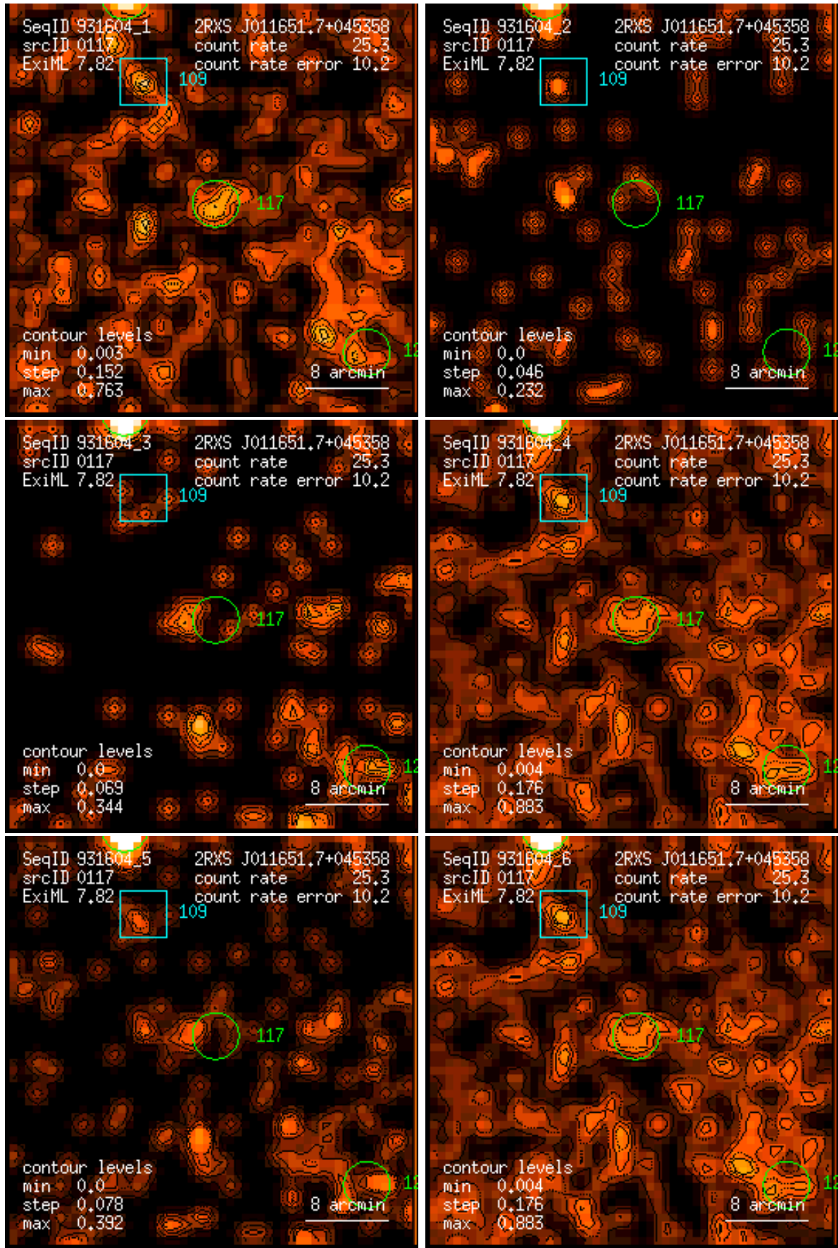
Figure 117: RASS 931604: detection 0117: band rate images, Gaussian filter: (1) PSPC channels 11 – 41, (2) 52 – 90, (3) 91 – 201, (4) 11 – 235, (5) 52 – 201, (6) 11 – 201. Broad band rates in counts/ks. Band rate contour levels in counts/ks/arcmin 2 .
