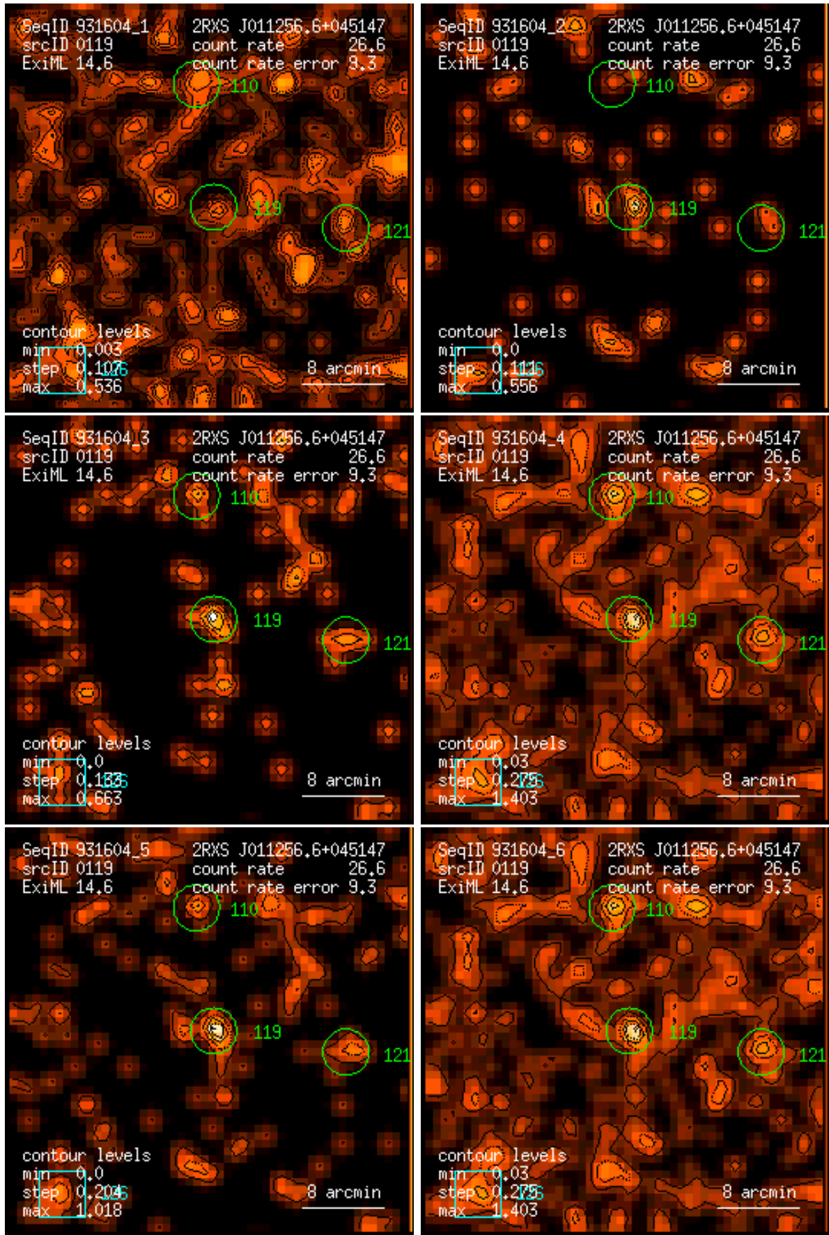
Figure 119: RASS 931604: detection 0119: band rate images, Gaussian filter: (1) PSPC channels 11 – 41, (2) 52 – 90, (3) 91 – 201, (4) 11 – 235, (5) 52 – 201, (6) 11 – 201. Broad band rates in counts/ks. Band rate contour levels in counts/ks/arcmin 2 .
