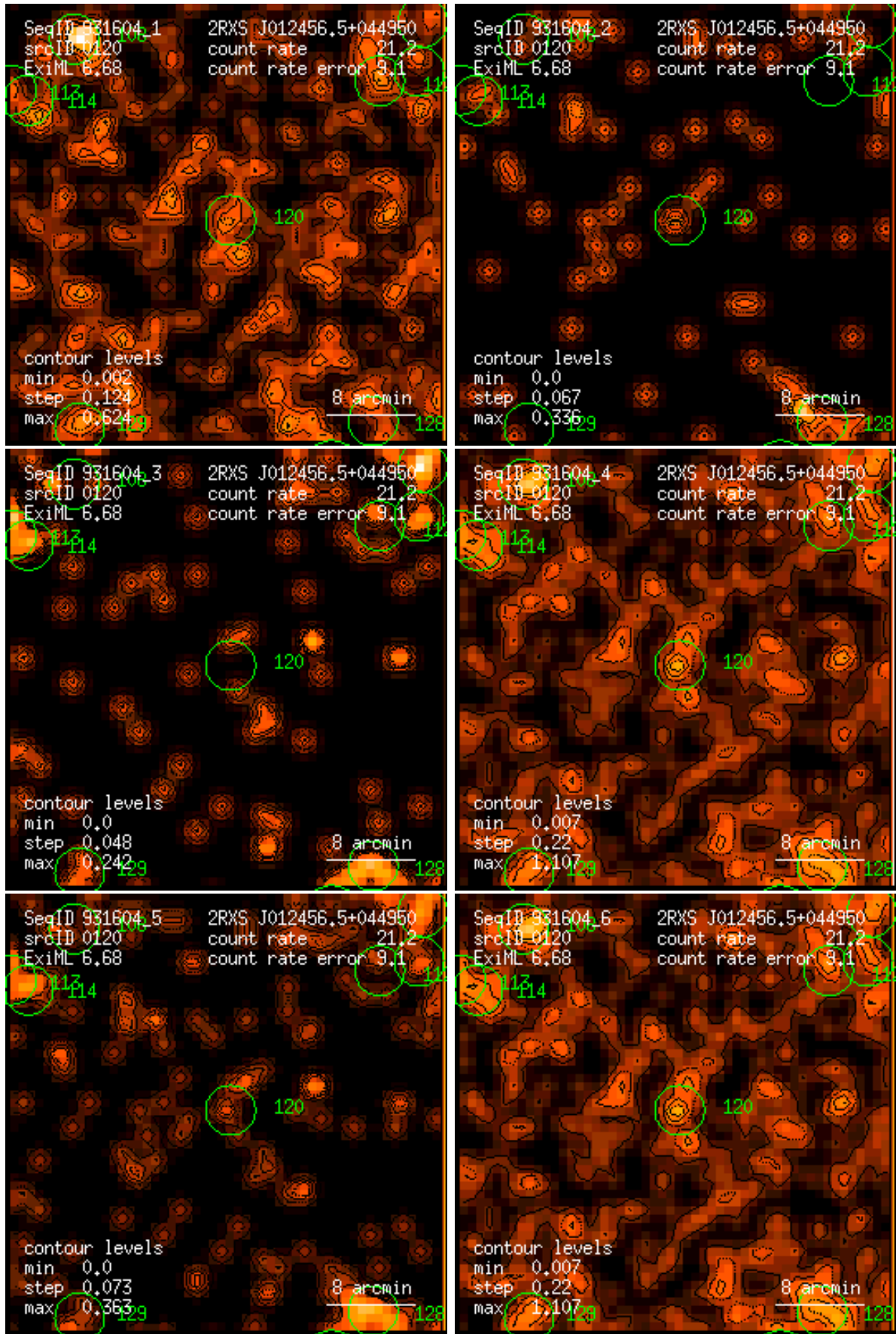
Figure 120: RASS 931604: detection 0120: band rate images, Gaussian filter: (1) PSPC channels 11 – 41, (2) 52 – 90, (3) 91 – 201, (4) 11 – 235, (5) 52 – 201, (6) 11 – 201. Broad band rates in counts/ks. Band rate contour levels in counts/ks/arcmin 2 .
