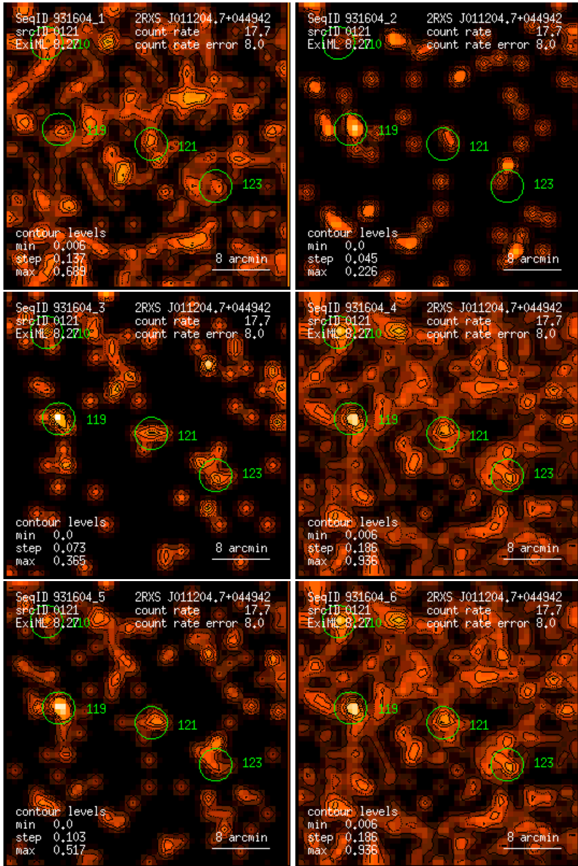
Figure 121: RASS 931604: detection 0121: band rate images, Gaussian filter: (1) PSPC channels 11 – 41, (2) 52 – 90, (3) 91 – 201, (4) 11 – 235, (5) 52 – 201, (6) 11 – 201. Broad band rates in counts/ks. Band rate contour levels in counts/ks/arcmin 2 .
