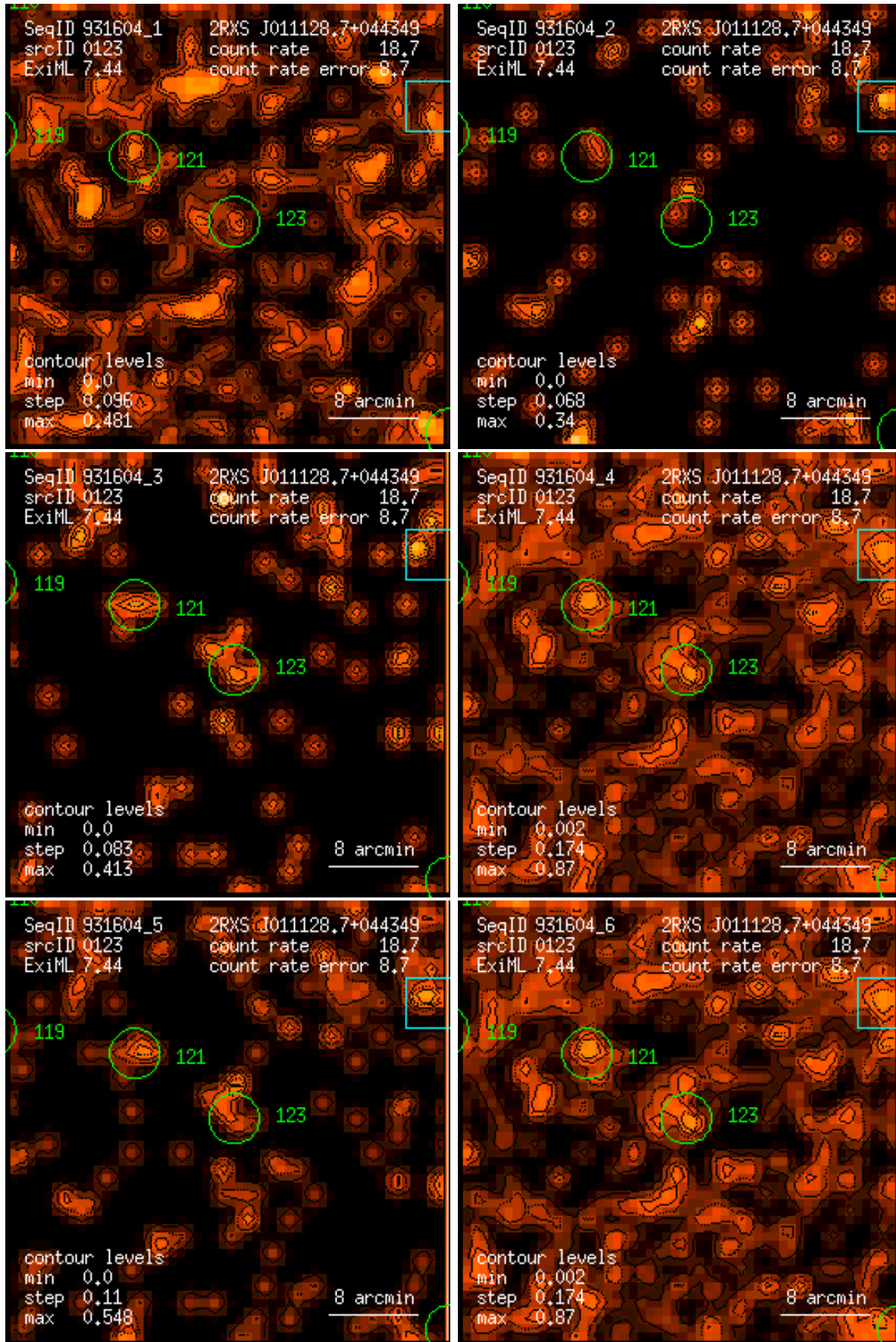
Figure 123: RASS 931604: detection 0123: band rate images, Gaussian filter: (1) PSPC channels 11 – 41, (2) 52 – 90, (3) 91 – 201, (4) 11 – 235, (5) 52 – 201, (6) 11 – 201. Broad band rates in counts/ks. Band rate contour levels in counts/ks/arcmin 2 .
