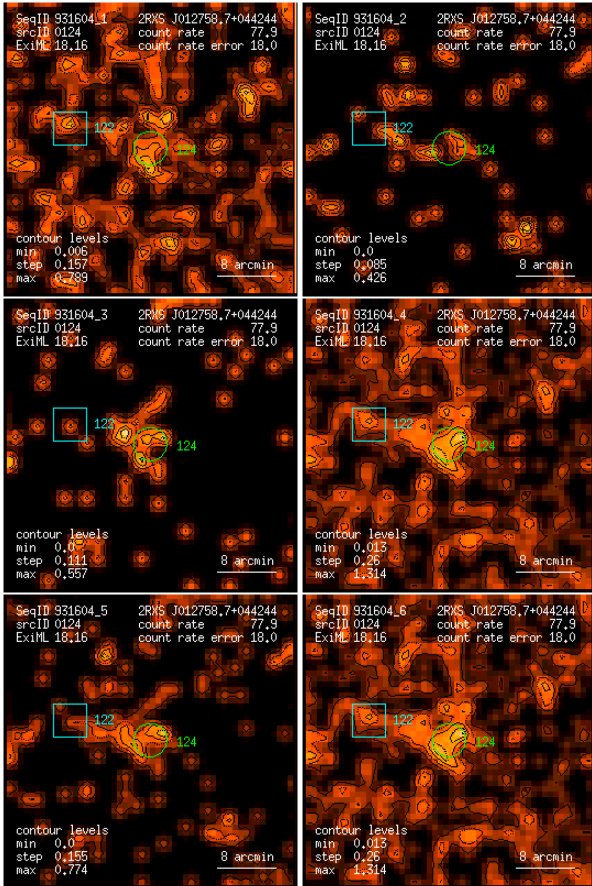
Figure 124: RASS 931604: detection 0124: band rate images, Gaussian filter: (1) PSPC channels 11 – 41, (2) 52 – 90, (3) 91 – 201, (4) 11 – 235, (5) 52 – 201, (6) 11 – 201. Broad band rates in counts/ks. Band rate contour levels in counts/ks/arcmin 2 .
