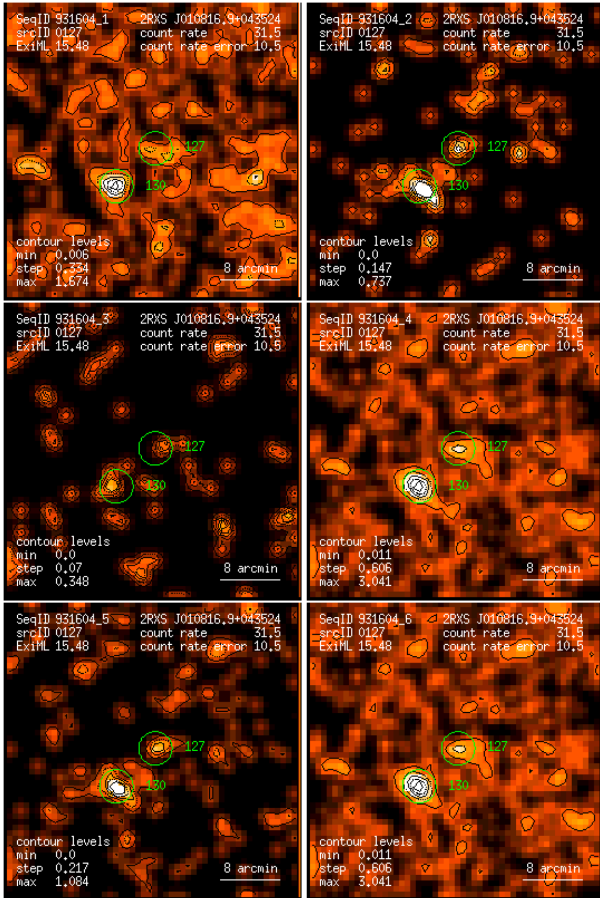
Figure 127: RASS 931604: detection 0127: band rate images, Gaussian filter: (1) PSPC channels 11 – 41, (2) 52 – 90, (3) 91 – 201, (4) 11 – 235, (5) 52 – 201, (6) 11 – 201. Broad band rates in counts/ks. Band rate contour levels in counts/ks/arcmin 2 .
