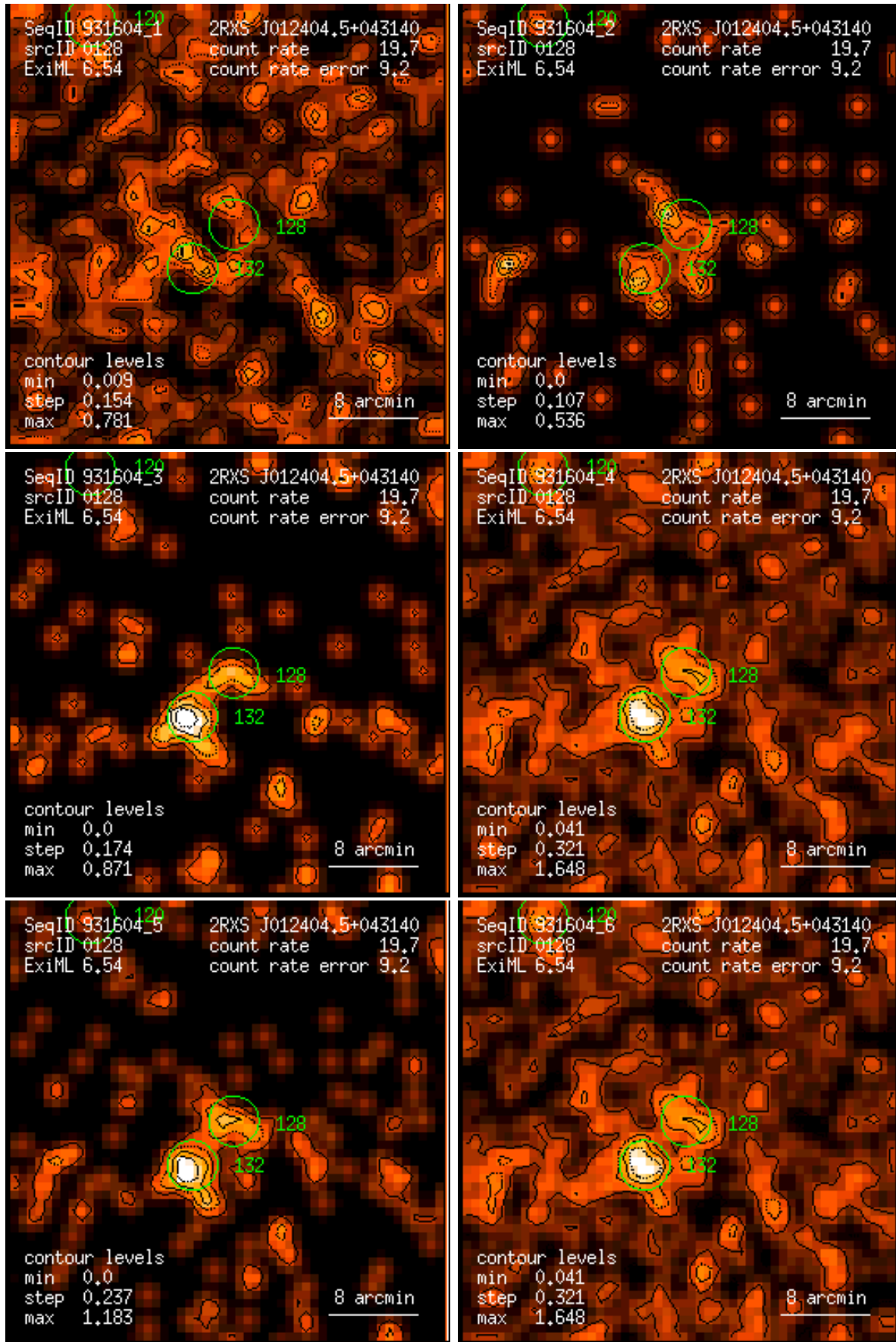
Figure 128: RASS 931604: detection 0128: band rate images, Gaussian filter: (1) PSPC channels 11 – 41, (2) 52 – 90, (3) 91 – 201, (4) 11 – 235, (5) 52 – 201, (6) 11 – 201. Broad band rates in counts/ks. Band rate contour levels in counts/ks/arcmin 2 .
