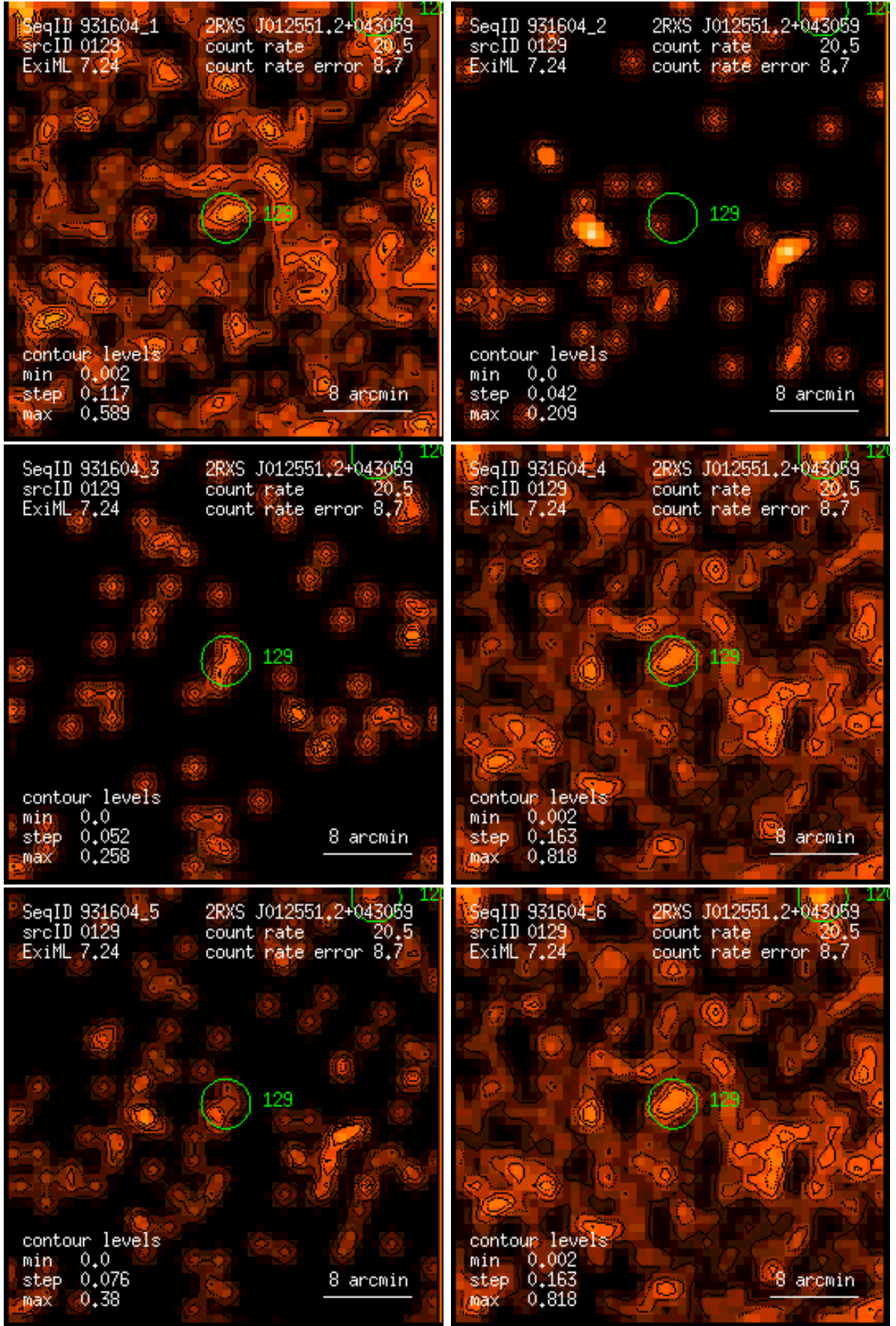
Figure 129: RASS 931604: detection 0129: band rate images, Gaussian filter: (1) PSPC channels 11 – 41, (2) 52 – 90, (3) 91 – 201, (4) 11 – 235, (5) 52 – 201, (6) 11 – 201. Broad band rates in counts/ks. Band rate contour levels in counts/ks/arcmin 2 .
