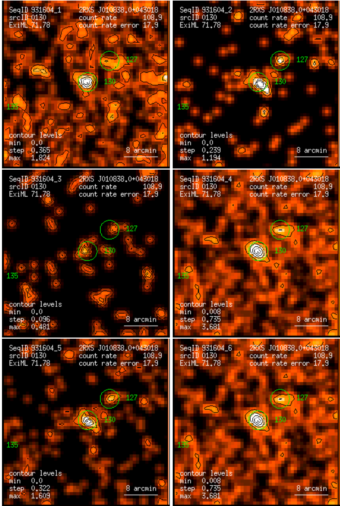
Figure 130: RASS 931604: detection 0130: band rate images, Gaussian filter: (1) PSPC channels 11 – 41, (2) 52 – 90, (3) 91 – 201, (4) 11 – 235, (5) 52 – 201, (6) 11 – 201. Broad band rates in counts/ks. Band rate contour levels in counts/ks/arcmin 2 .
