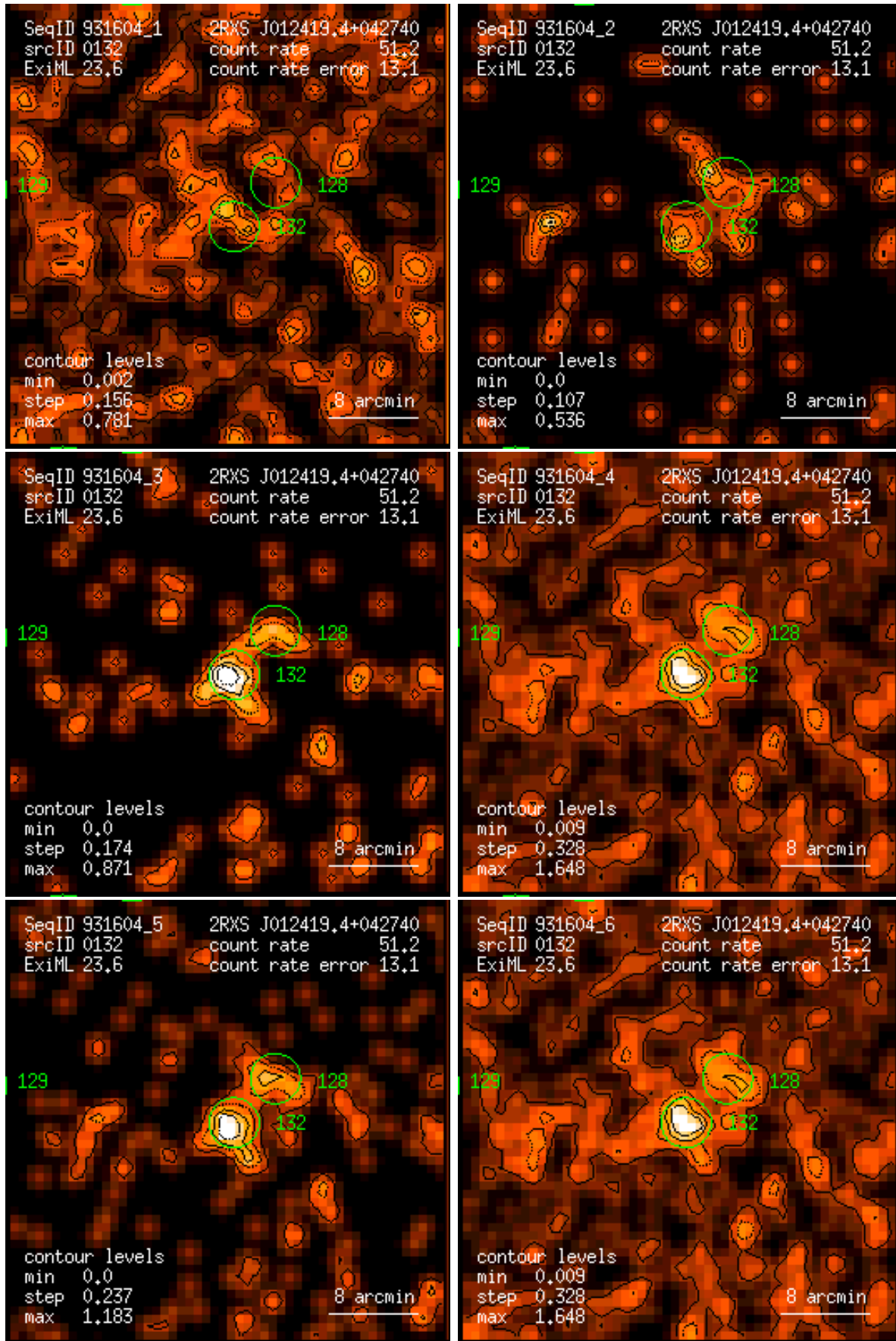
Figure 132: RASS 931604: detection 0132: band rate images, Gaussian filter: (1) PSPC channels 11 – 41, (2) 52 – 90, (3) 91 – 201, (4) 11 – 235, (5) 52 – 201, (6) 11 – 201. Broad band rates in counts/ks. Band rate contour levels in counts/ks/arcmin 2 .
