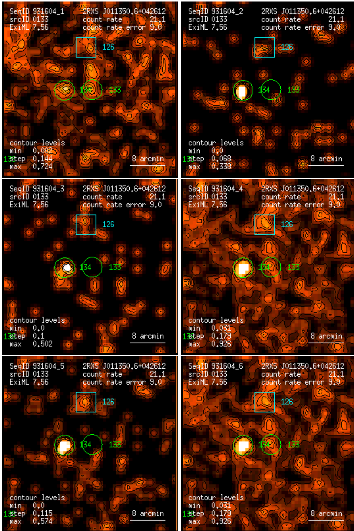
Figure 133: RASS 931604: detection 0133: band rate images, Gaussian filter: (1) PSPC channels 11 – 41, (2) 52 – 90, (3) 91 – 201, (4) 11 – 235, (5) 52 – 201, (6) 11 – 201. Broad band rates in counts/ks. Band rate contour levels in counts/ks/arcmin 2 .
