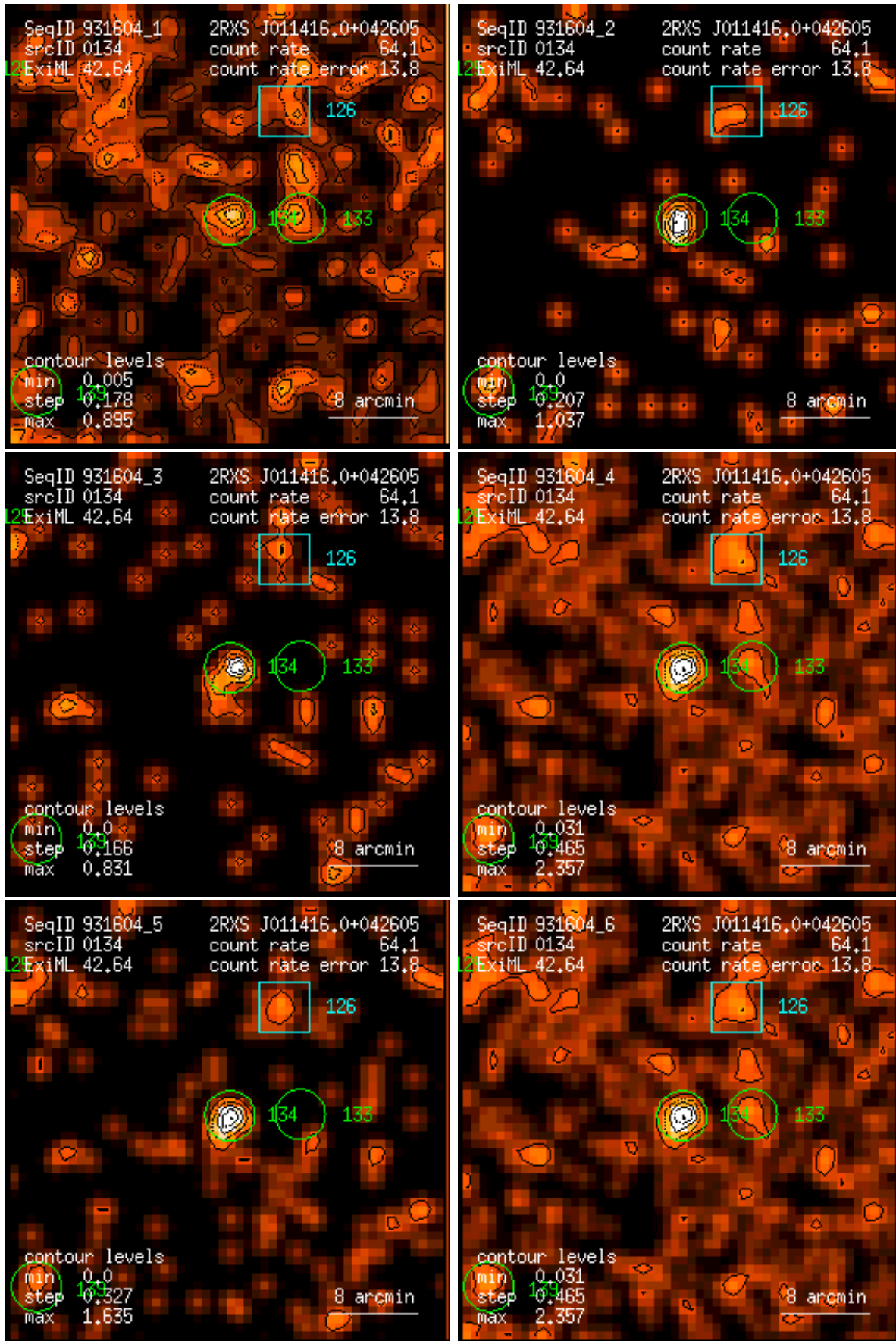
Figure 134: RASS 931604: detection 0134: band rate images, Gaussian filter: (1) PSPC channels 11 – 41, (2) 52 – 90, (3) 91 – 201, (4) 11 – 235, (5) 52 – 201, (6) 11 – 201. Broad band rates in counts/ks. Band rate contour levels in counts/ks/arcmin 2 .
