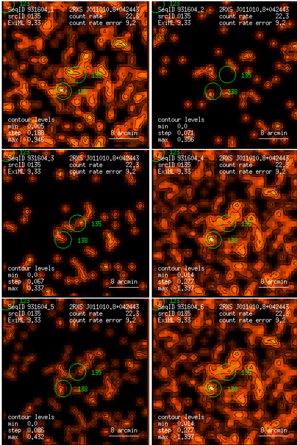
Figure 135: RASS 931604: detection 0135: band rate images, Gaussian filter: (1) PSPC channels 11 – 41, (2) 52 – 90, (3) 91 – 201, (4) 11 – 235, (5) 52 – 201, (6) 11 – 201. Broad band rates in counts/ks. Band rate contour levels in counts/ks/arcmin 2 .
