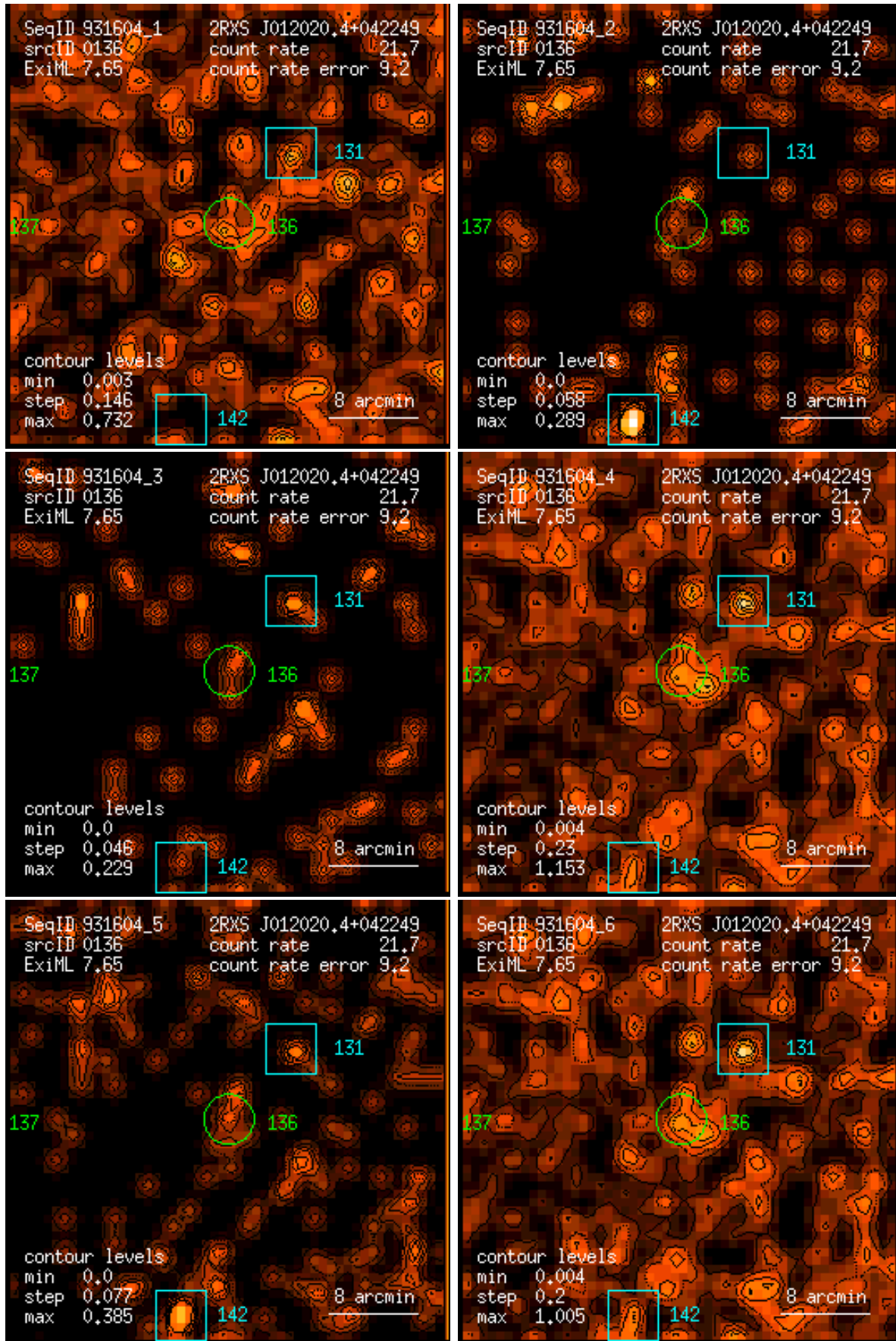
Figure 136: RASS 931604: detection 0136: band rate images, Gaussian filter: (1) PSPC channels 11 – 41, (2) 52 – 90, (3) 91 – 201, (4) 11 – 235, (5) 52 – 201, (6) 11 – 201. Broad band rates in counts/ks. Band rate contour levels in counts/ks/arcmin 2 .
