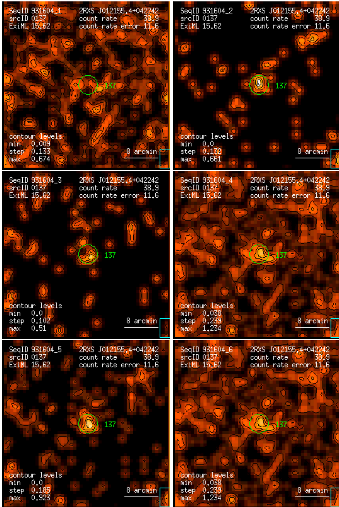
Figure 137: RASS 931604: detection 0137: band rate images, Gaussian filter: (1) PSPC channels 11 – 41, (2) 52 – 90, (3) 91 – 201, (4) 11 – 235, (5) 52 – 201, (6) 11 – 201. Broad band rates in counts/ks. Band rate contour levels in counts/ks/arcmin 2 .
