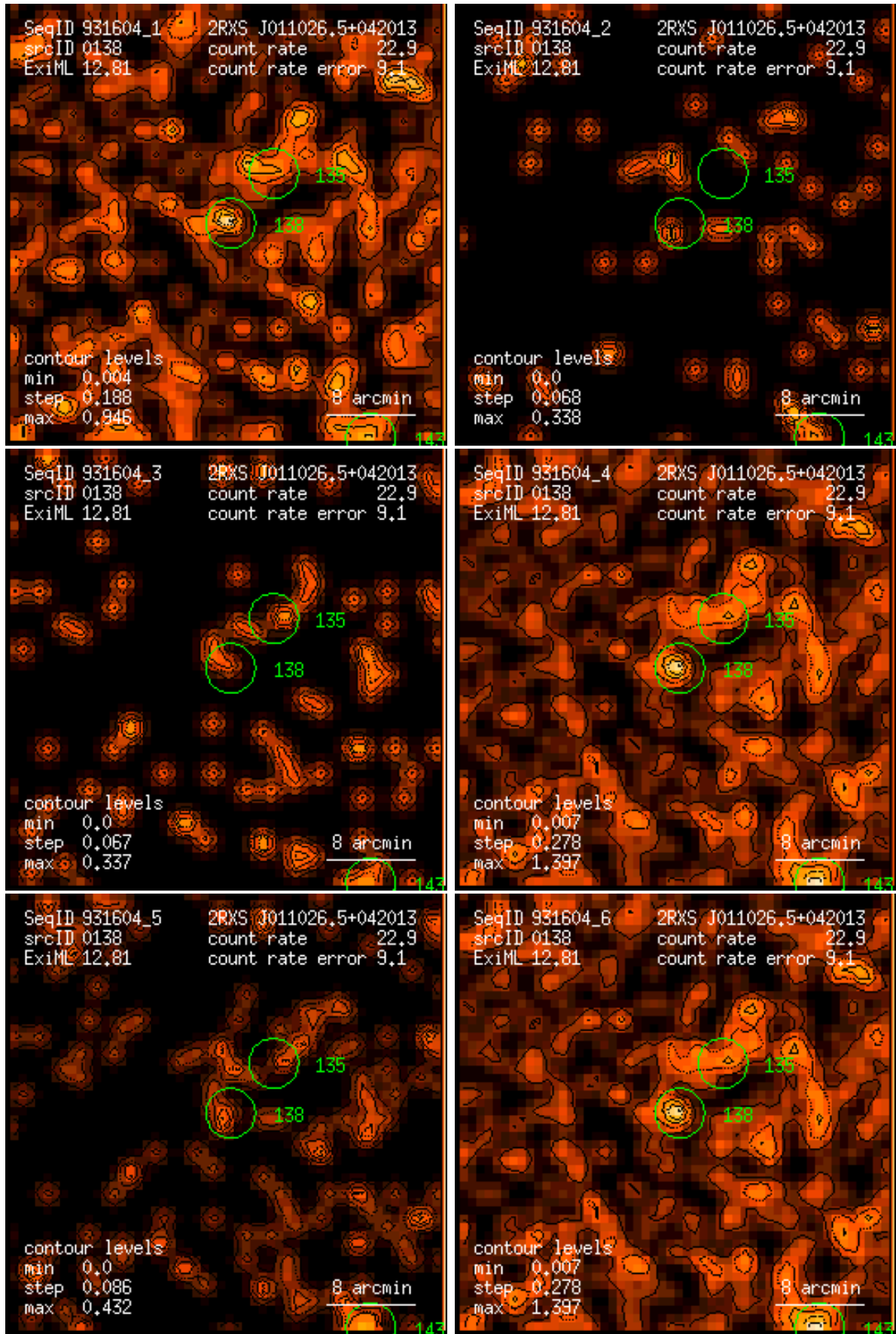
Figure 138: RASS 931604: detection 0138: band rate images, Gaussian filter: (1) PSPC channels 11 – 41, (2) 52 – 90, (3) 91 – 201, (4) 11 – 235, (5) 52 – 201, (6) 11 – 201. Broad band rates in counts/ks. Band rate contour levels in counts/ks/arcmin 2 .
