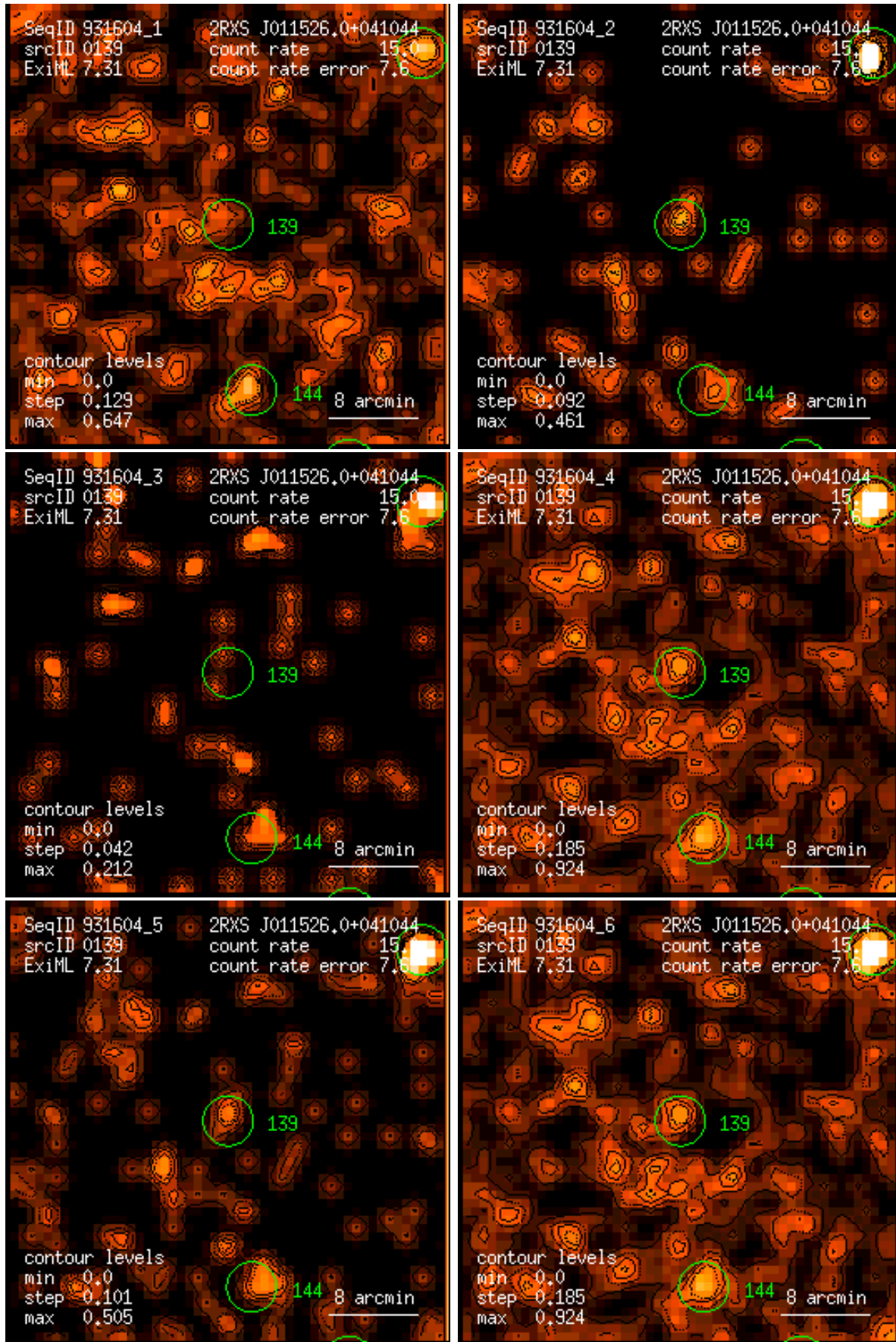
Figure 139: RASS 931604: detection 0139: band rate images, Gaussian filter: (1) PSPC channels 11 – 41, (2) 52 – 90, (3) 91 – 201, (4) 11 – 235, (5) 52 – 201, (6) 11 – 201. Broad band rates in counts/ks. Band rate contour levels in counts/ks/arcmin 2 .
