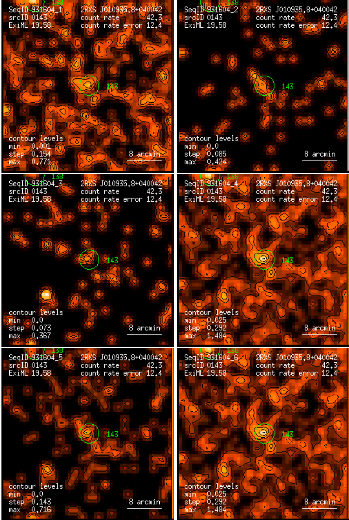
Figure 143: RASS 931604: detection 0143: band rate images, Gaussian filter: (1) PSPC channels 11 – 41, (2) 52 – 90, (3) 91 – 201, (4) 11 – 235, (5) 52 – 201, (6) 11 – 201. Broad band rates in counts/ks. Band rate contour levels in counts/ks/arcmin 2 .
