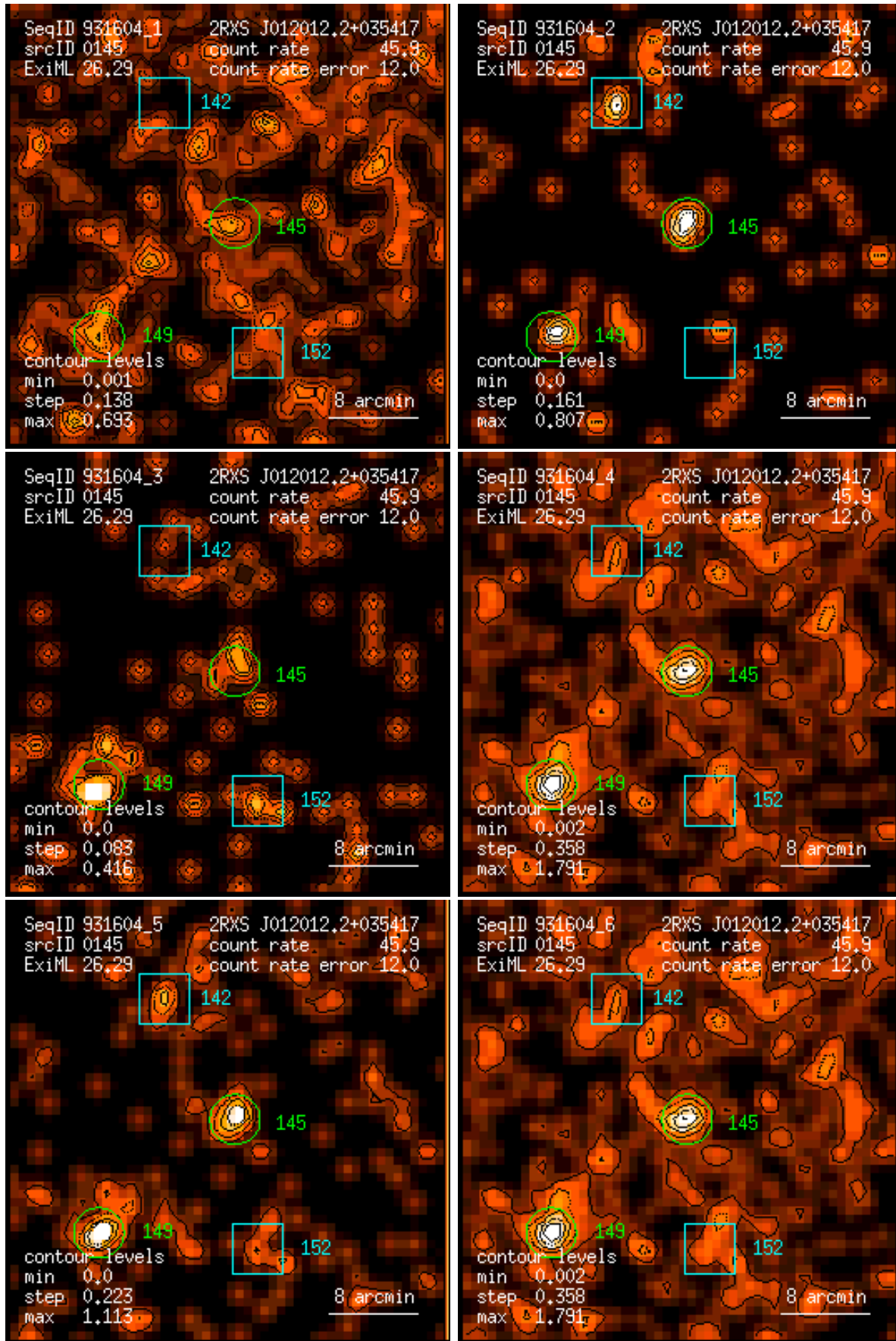
Figure 145: RASS 931604: detection 0145: band rate images, Gaussian filter: (1) PSPC channels 11 – 41, (2) 52 – 90, (3) 91 – 201, (4) 11 – 235, (5) 52 – 201, (6) 11 – 201. Broad band rates in counts/ks. Band rate contour levels in counts/ks/arcmin 2 .
