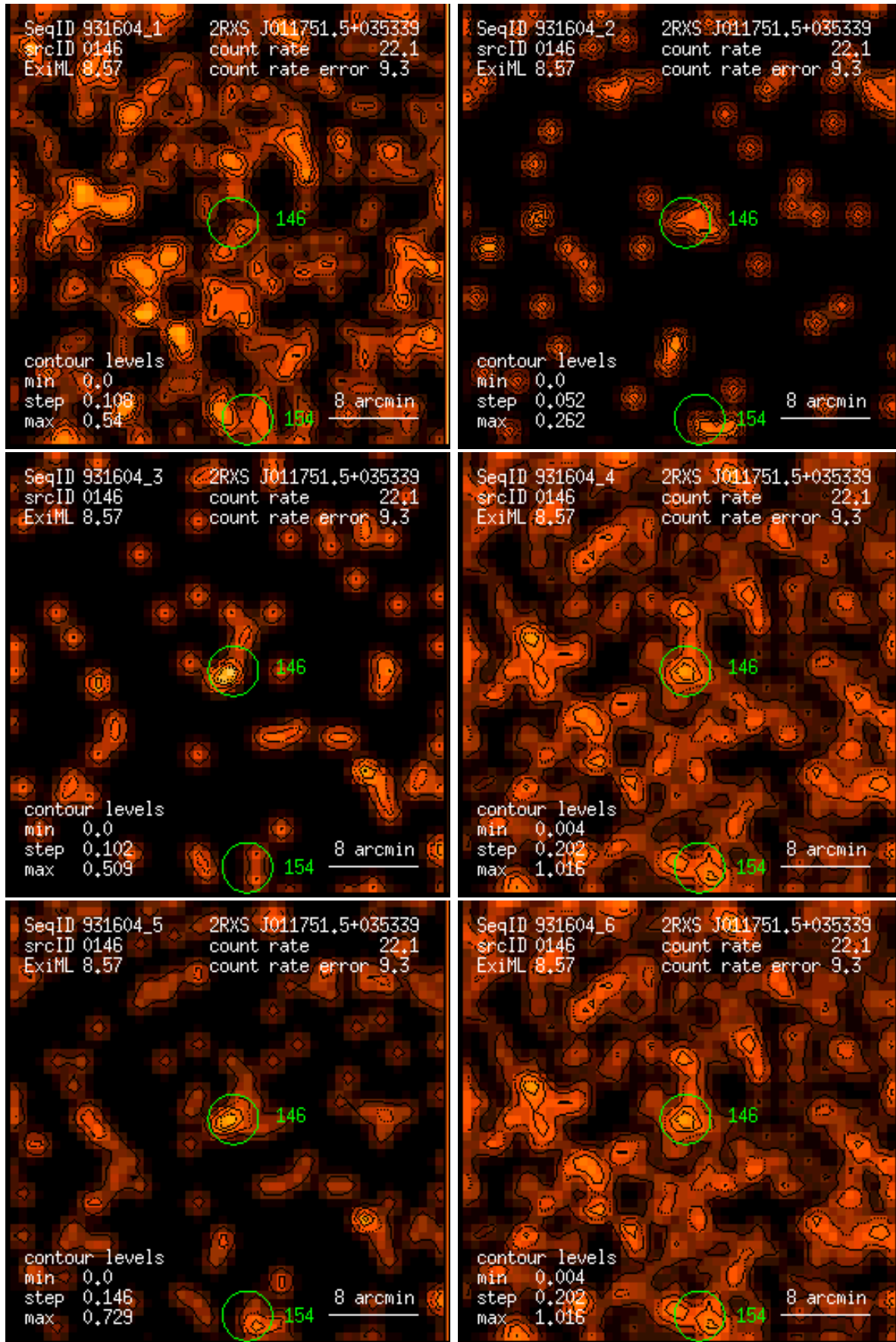
Figure 146: RASS 931604: detection 0146: band rate images, Gaussian filter: (1) PSPC channels 11 – 41, (2) 52 – 90, (3) 91 – 201, (4) 11 – 235, (5) 52 – 201, (6) 11 – 201. Broad band rates in counts/ks. Band rate contour levels in counts/ks/arcmin 2 .
