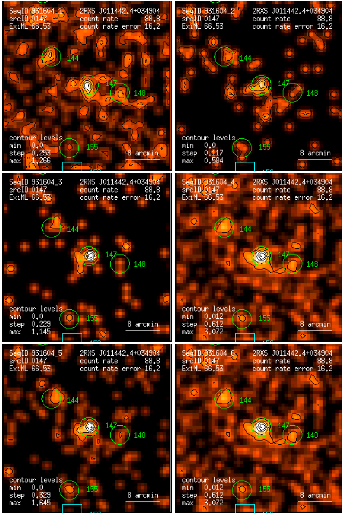
Figure 147: RASS 931604: detection 0147: band rate images, Gaussian filter: (1) PSPC channels 11 – 41, (2) 52 – 90, (3) 91 – 201, (4) 11 – 235, (5) 52 – 201, (6) 11 – 201. Broad band rates in counts/ks. Band rate contour levels in counts/ks/arcmin 2 .
