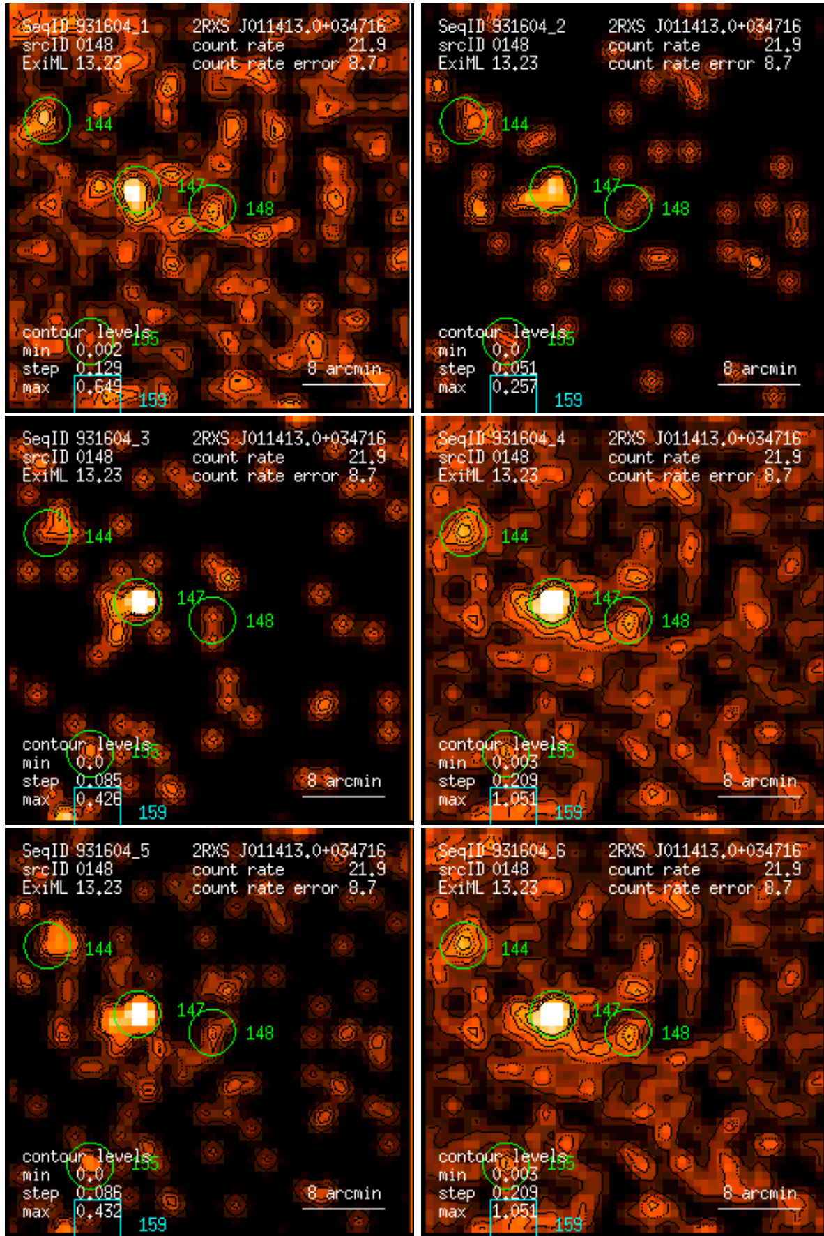
Figure 148: RASS 931604: detection 0148: band rate images, Gaussian filter: (1) PSPC channels 11 – 41, (2) 52 – 90, (3) 91 – 201, (4) 11 – 235, (5) 52 – 201, (6) 11 – 201. Broad band rates in counts/ks. Band rate contour levels in counts/ks/arcmin 2 .
