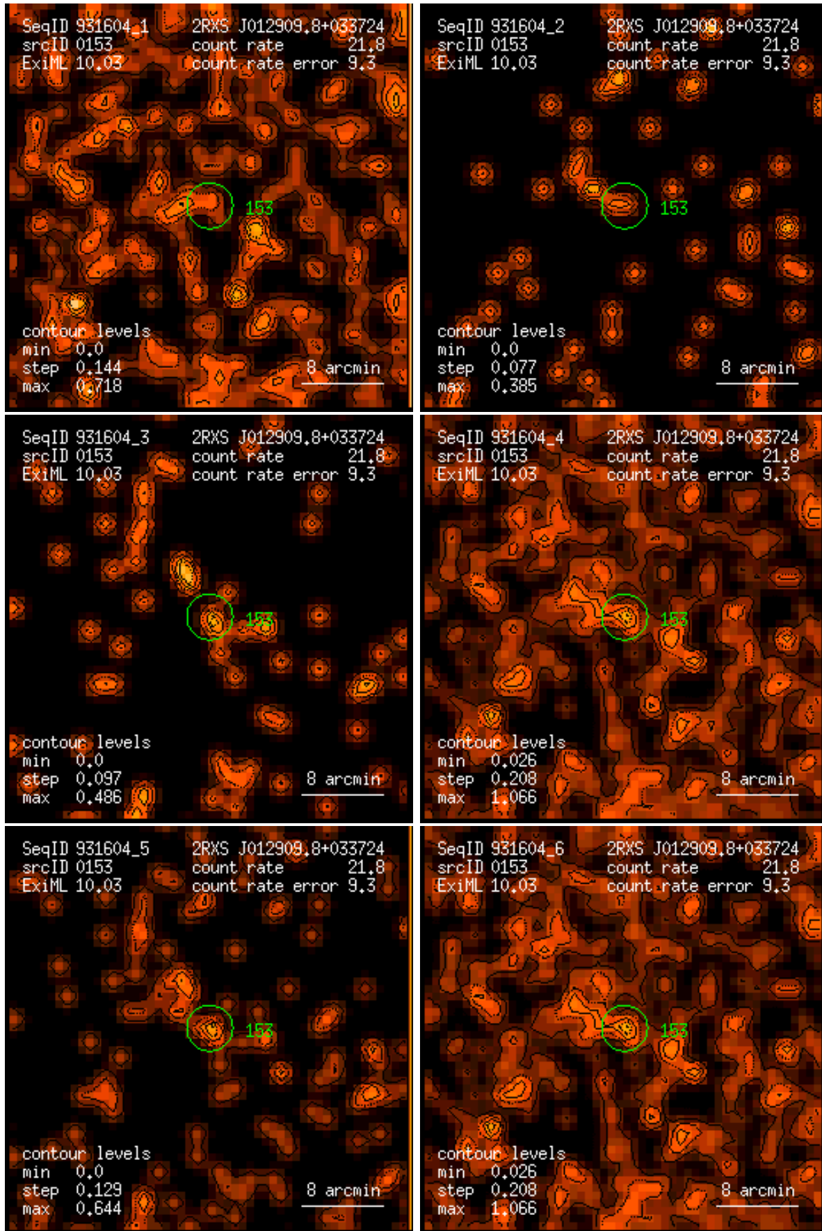
Figure 153: RASS 931604: detection 0153: band rate images, Gaussian filter: (1) PSPC channels 11 – 41, (2) 52 – 90, (3) 91 – 201, (4) 11 – 235, (5) 52 – 201, (6) 11 – 201. Broad band rates in counts/ks. Band rate contour levels in counts/ks/arcmin 2 .
