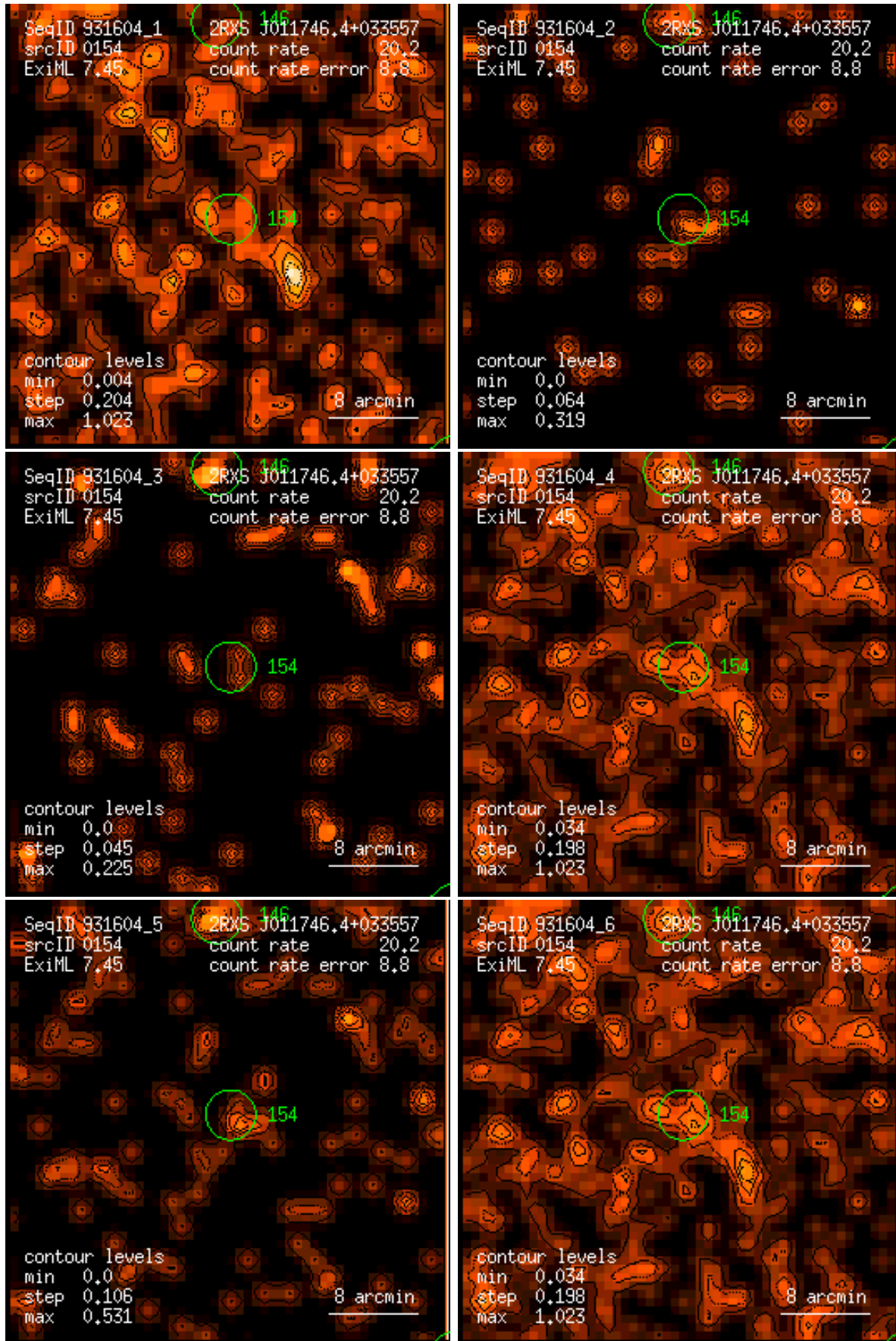
Figure 154: RASS 931604: detection 0154: band rate images, Gaussian filter: (1) PSPC channels 11 – 41, (2) 52 – 90, (3) 91 – 201, (4) 11 – 235, (5) 52 – 201, (6) 11 – 201. Broad band rates in counts/ks. Band rate contour levels in counts/ks/arcmin 2 .
