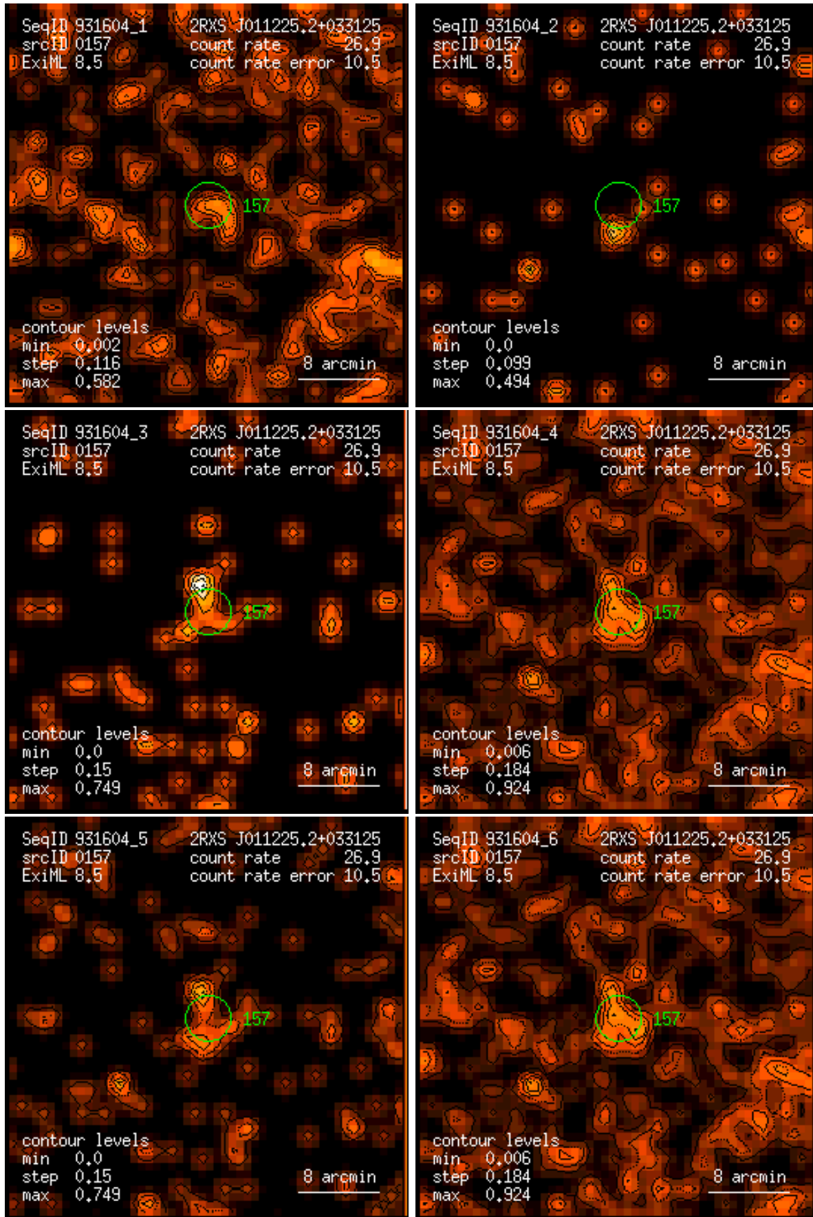
Figure 157: RASS 931604: detection 0157: band rate images, Gaussian filter: (1) PSPC channels 11 – 41, (2) 52 – 90, (3) 91 – 201, (4) 11 – 235, (5) 52 – 201, (6) 11 – 201. Broad band rates in counts/ks. Band rate contour levels in counts/ks/arcmin 2 .
