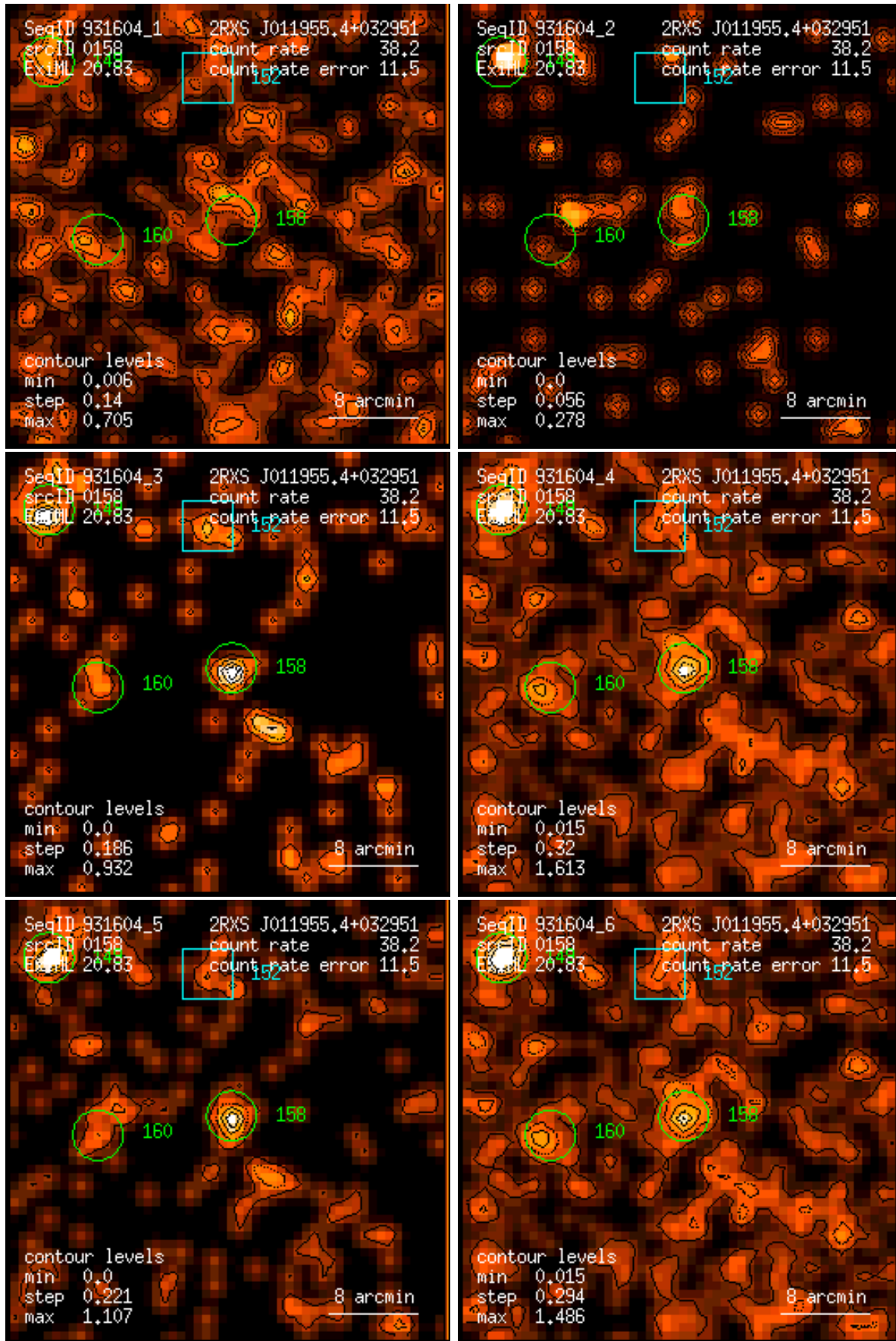
Figure 158: RASS 931604: detection 0158: band rate images, Gaussian filter: (1) PSPC channels 11 – 41, (2) 52 – 90, (3) 91 – 201, (4) 11 – 235, (5) 52 – 201, (6) 11 – 201. Broad band rates in counts/ks. Band rate contour levels in counts/ks/arcmin 2 .
