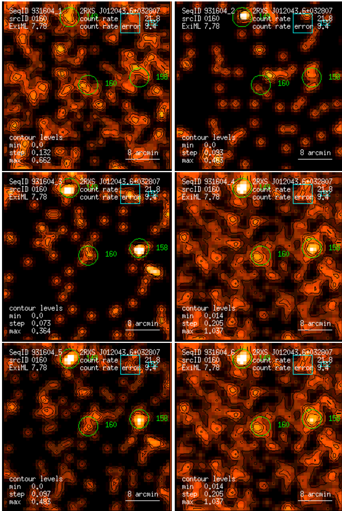
Figure 160: RASS 931604: detection 0160: band rate images, Gaussian filter: (1) PSPC channels 11 – 41, (2) 52 – 90, (3) 91 – 201, (4) 11 – 235, (5) 52 – 201, (6) 11 – 201. Broad band rates in counts/ks. Band rate contour levels in counts/ks/arcmin 2 .
