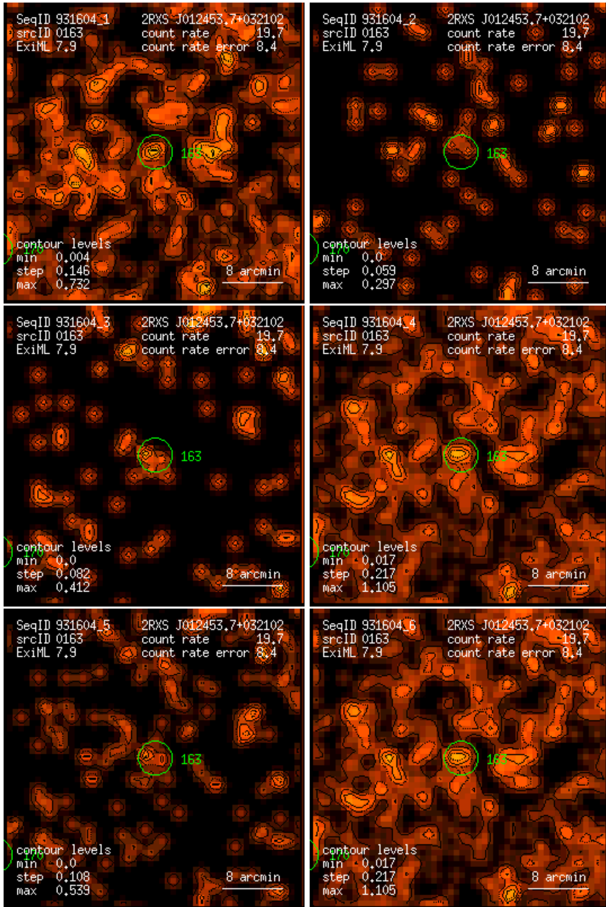
Figure 163: RASS 931604: detection 0163: band rate images, Gaussian filter: (1) PSPC channels 11 – 41, (2) 52 – 90, (3) 91 – 201, (4) 11 – 235, (5) 52 – 201, (6) 11 – 201. Broad band rates in counts/ks. Band rate contour levels in counts/ks/arcmin 2 .
